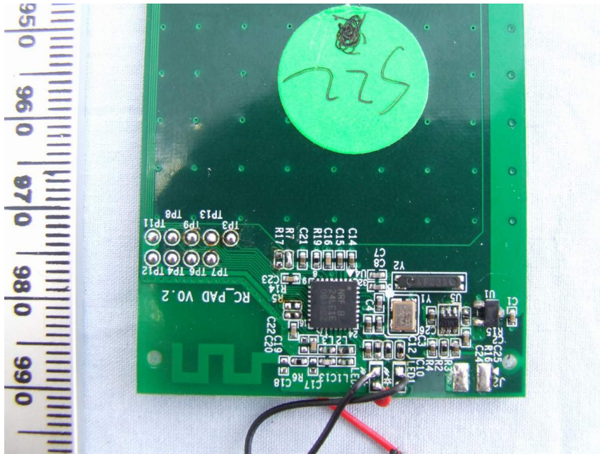
PCB View 2
