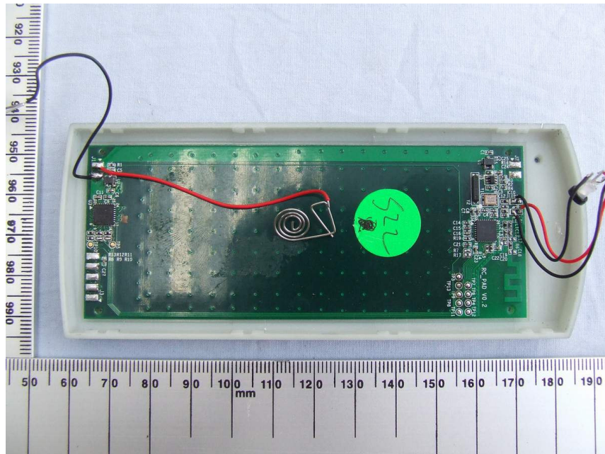
Uncovered View
