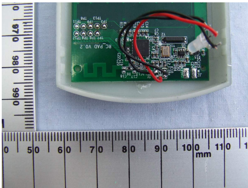
PCB View 3
