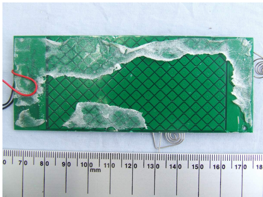
PCB View 1
