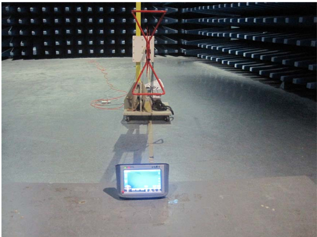
Radiated Spurious Emissions Test Setup (30MHz-1GHz)
