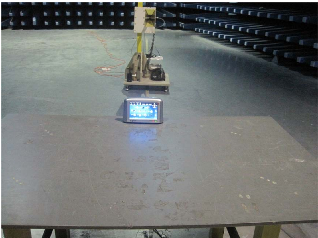
Radiated Spurious Emissions Test Setup (Above 1GHz)
