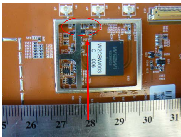
(Switch Circuit)
