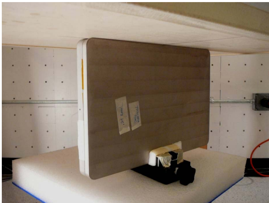
Right Touch to Flat Phantom Setup Photo
