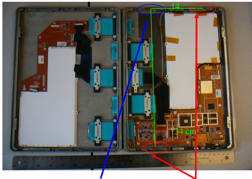
(Bluetooth Antenna Location)
