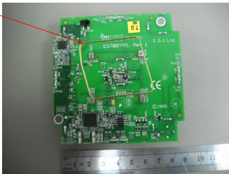
Photograph 7.5.1 RFID antenna assembly
