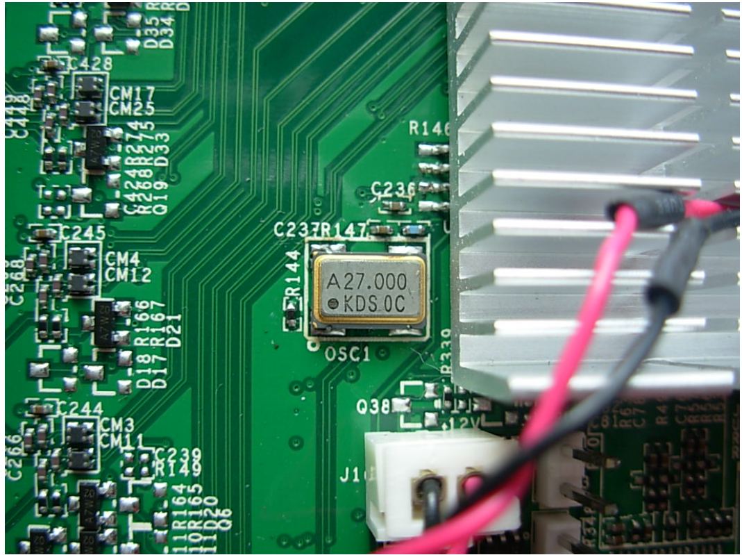
FIGURE 3 GRAPHIC CARD (M/N: FI5400E-2G8H1GF(8-HDMI)) CRYSTAL ON MAIN BOARD
