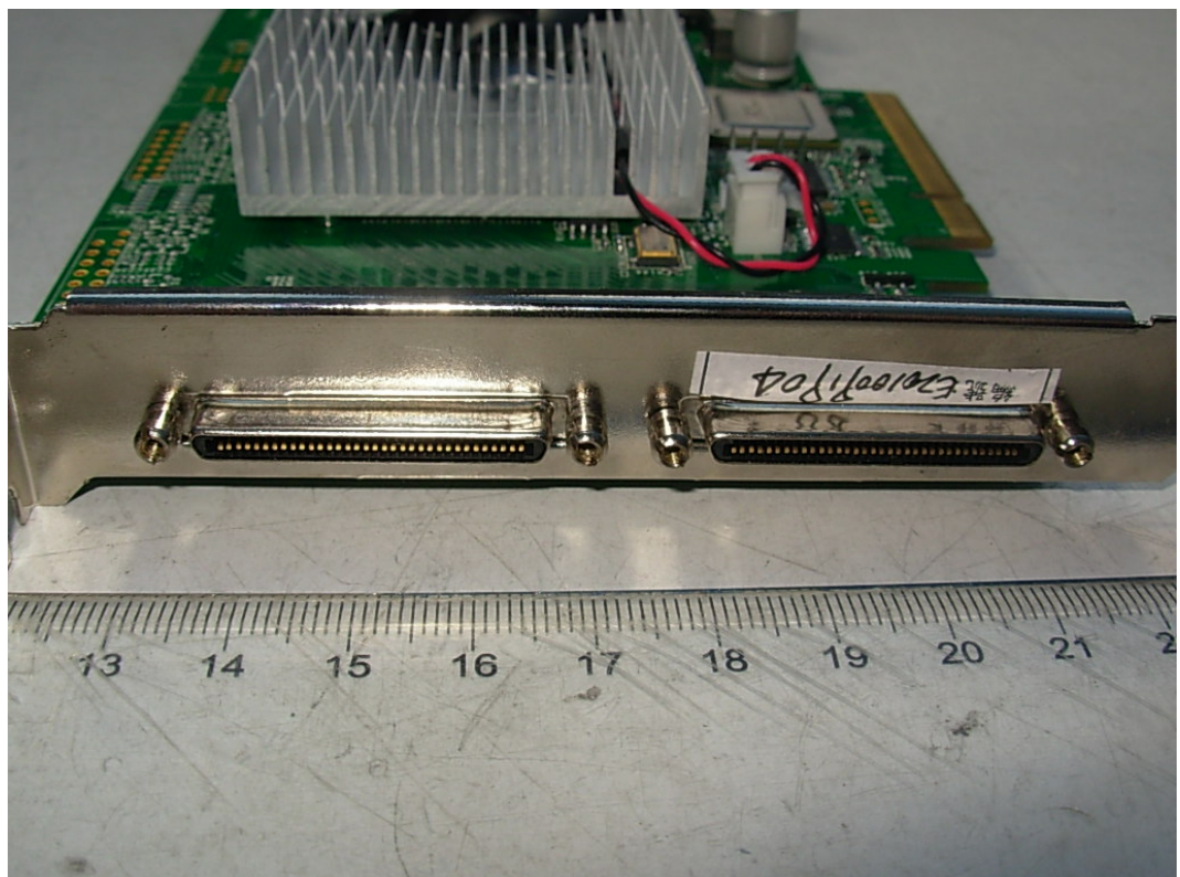
FIGURE 2 GRAPHIC CARD (M/N: FI5400E-2G8H1GF(8-HDMI)) MAIN BOARD SIGNAL PORTS
