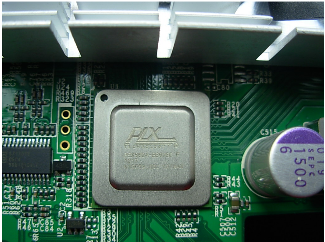
FIGURE 5 GRAPHIC CARD (M/N: FI5400E-2G8H1GF(8-HDMI)) CHIP 2 ON MAIN BOARD
