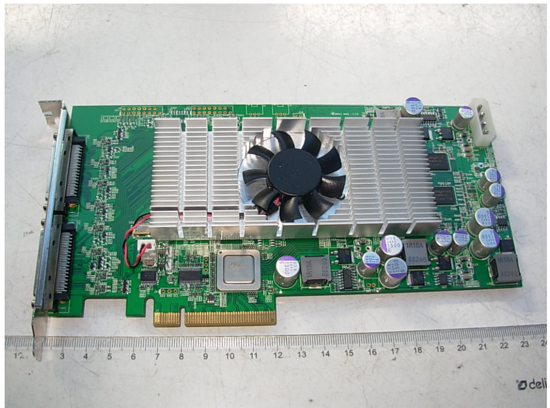
FIGURE 1 GRAPHIC CARD (M/N: FI5400E-2G8H1GF(8-HDMI)) MAIN BOARD (FRONT VIEW)
