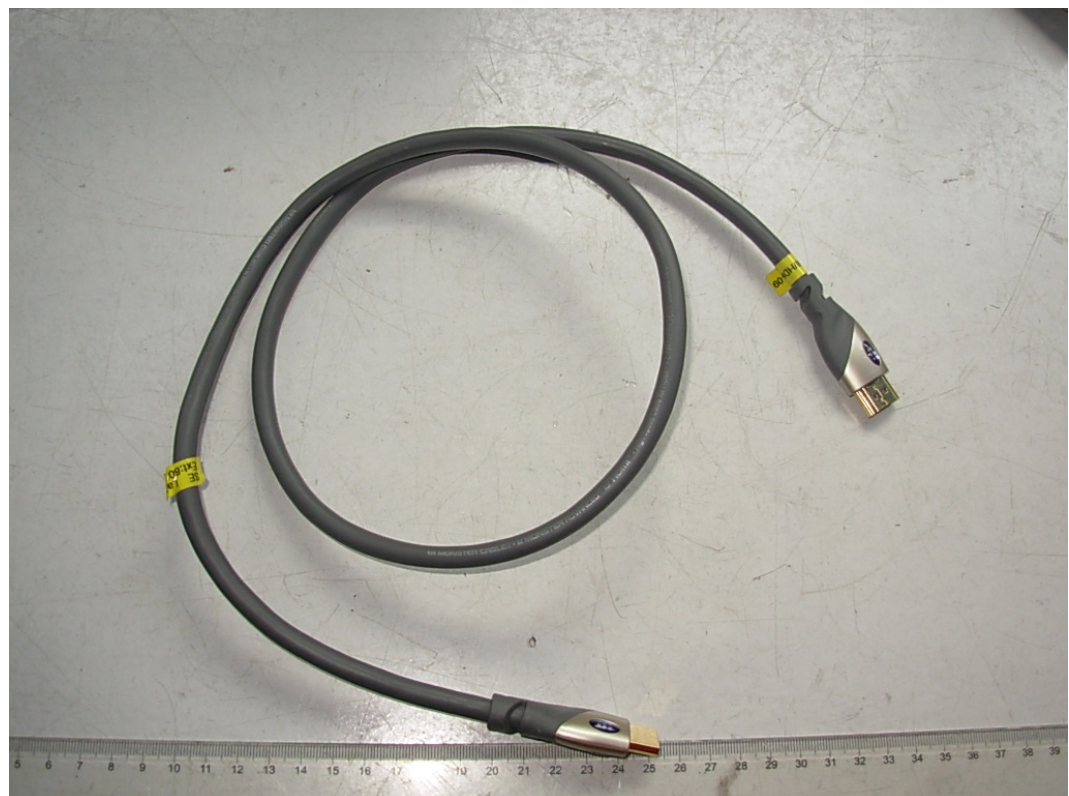
FIGURE 4 GRAPHIC CARD (M/N: FI5400E-2G8H1GF(8-HDMI)) HDMI CABLE
