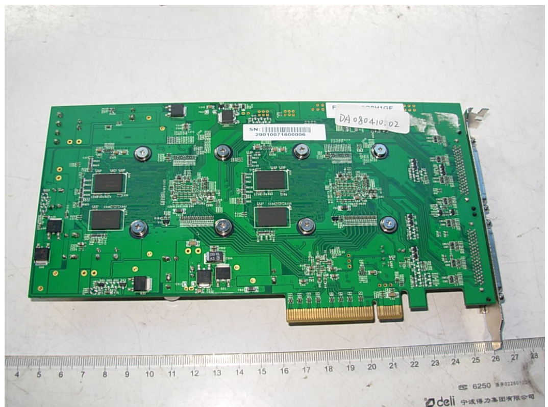
FIGURE 2 GRAPHIC CARD (M/N: FI5400E-2G8H1GF(8-HDMI)) MAIN BOARD (BACK VIEW)
