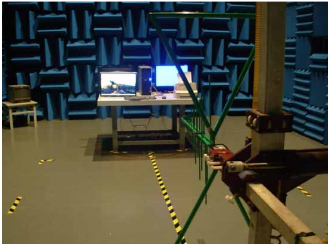
SETUP WITH MAXIMUM DETECTED EMISSION AT VERTICAL POLARIZATION (TEST MODE: HDMI 1280*1024P)
