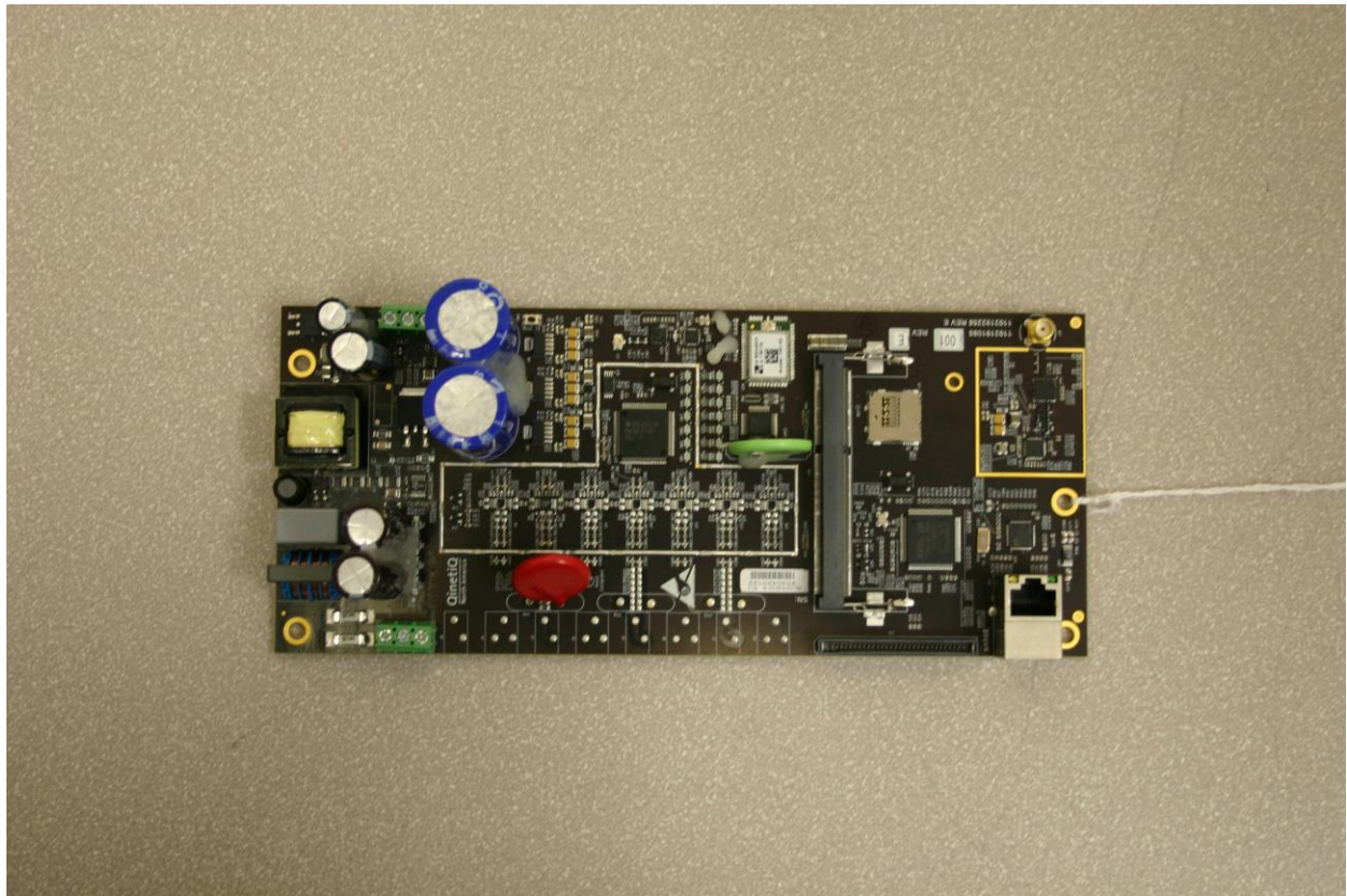
Photograph 9. Collector – PCB – Top
