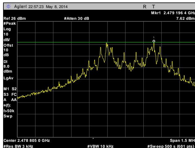
Plot 29. Peak Power Spectral Density, High Channel
