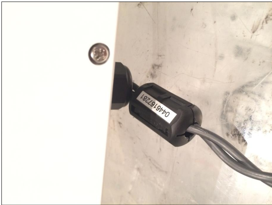
Photograph 3. Radiated Emissions, Test Setup, Ferrite Model Number
