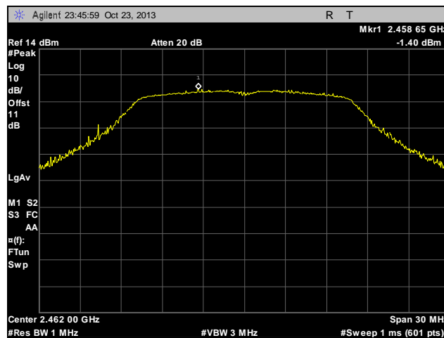
Plot 88. Peak Power Spectral Density, Determination, High Channel, 802.11g
