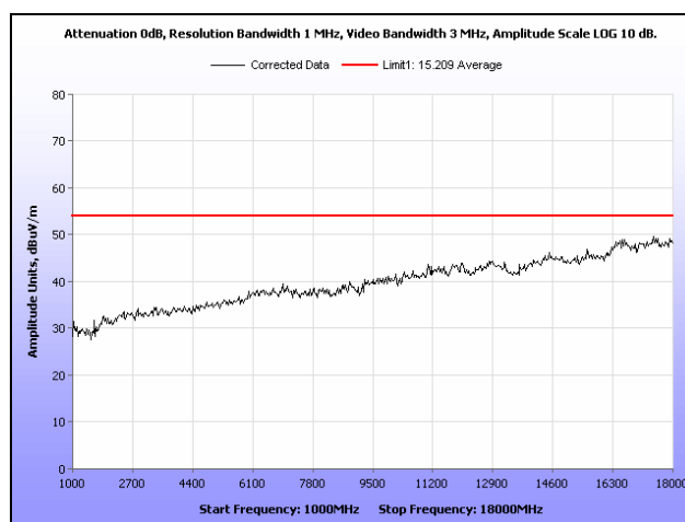
Plot 50. Radiated Spurious Emissions, High Channel, 802.11n, 1 GHz – 18 GHz, Peak under Average
