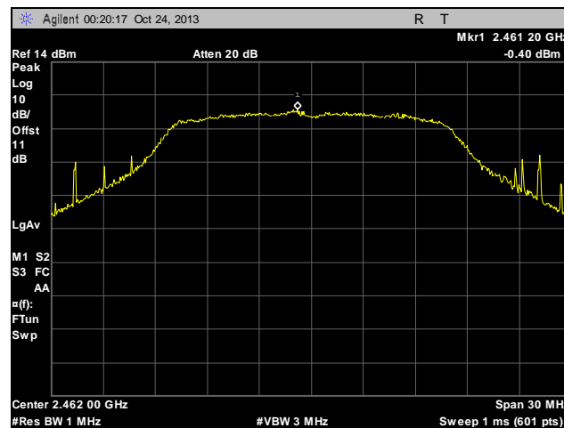
Plot 94. Peak Power Spectral Density, Determination, High Channel, 802.11n
