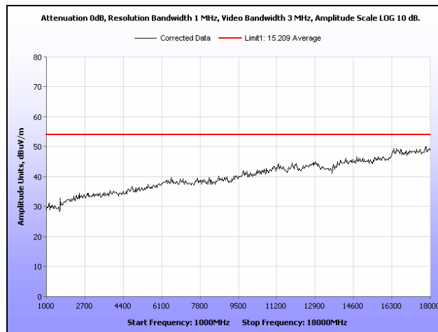
Plot 44. Radiated Spurious Emissions, High Channel, 802.11g, 1 GHz – 18 GHz, Peak under Average
