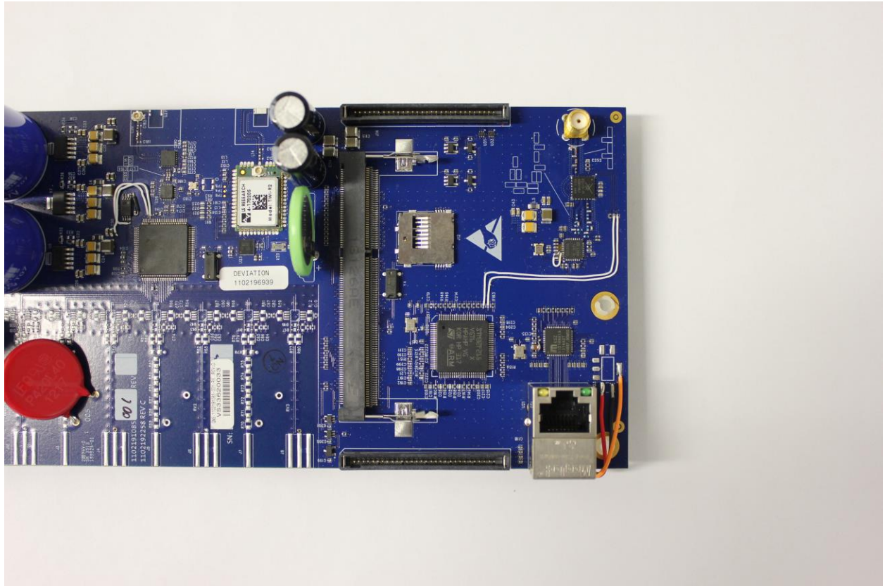
Photograph 3. Collector – Board – Close Up 2 of 2
