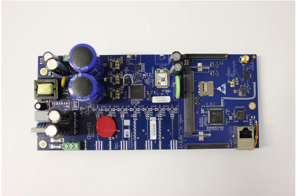
Photograph 4. Collector – Board – Front
