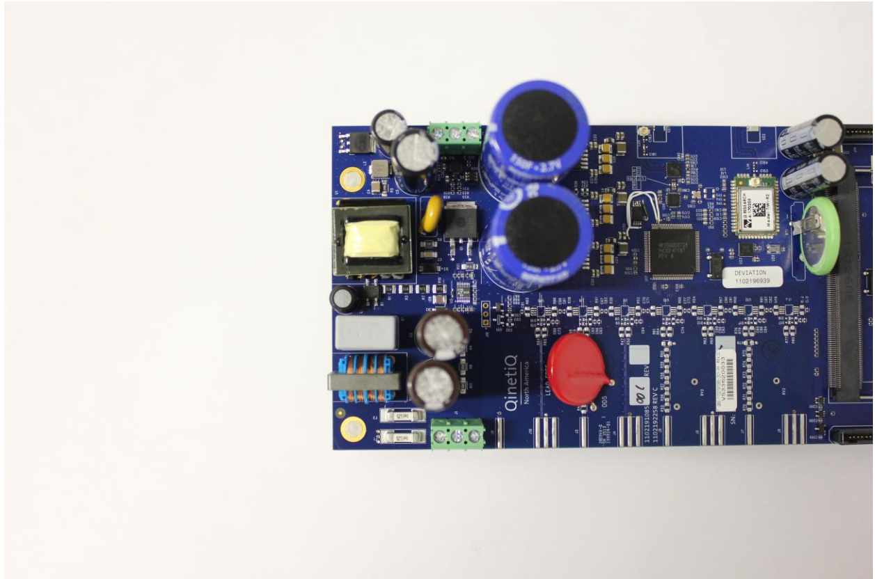
Photograph 2. Collector – Board – Close Up 1 of 2
