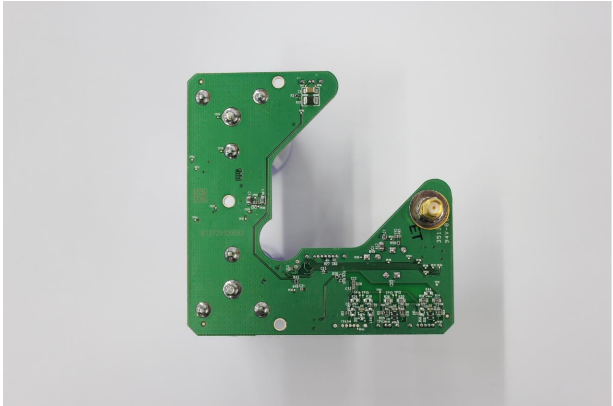
Photograph 1. Feeder Meter Sensor – Board – Back
