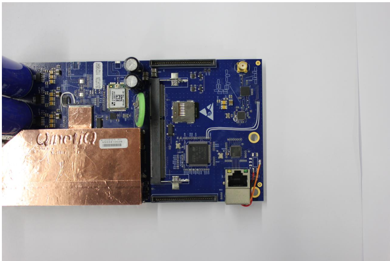
Photograph 5. Transformer Meter – Board Shielded – Close Up 2 of 2
