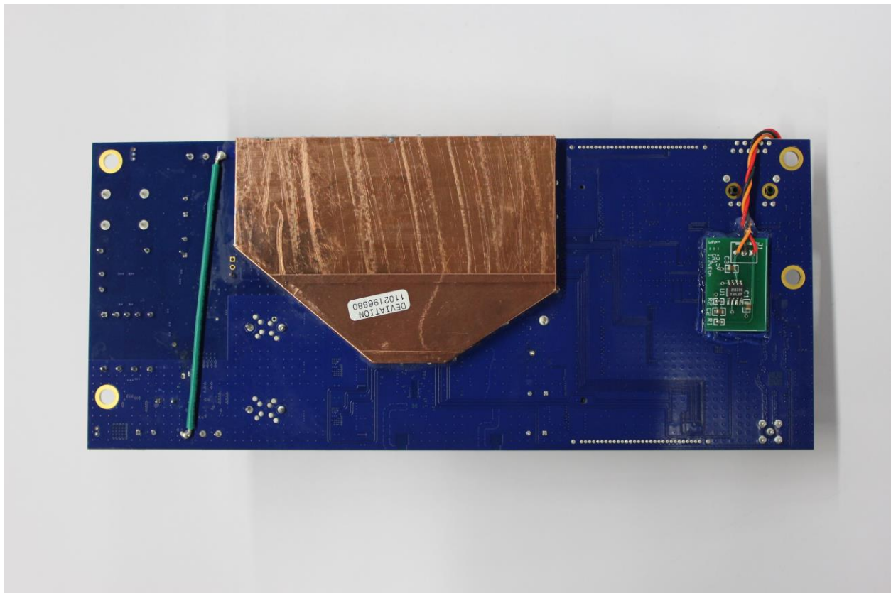
Photograph 3. Transformer Meter – Board Shielded - Back
