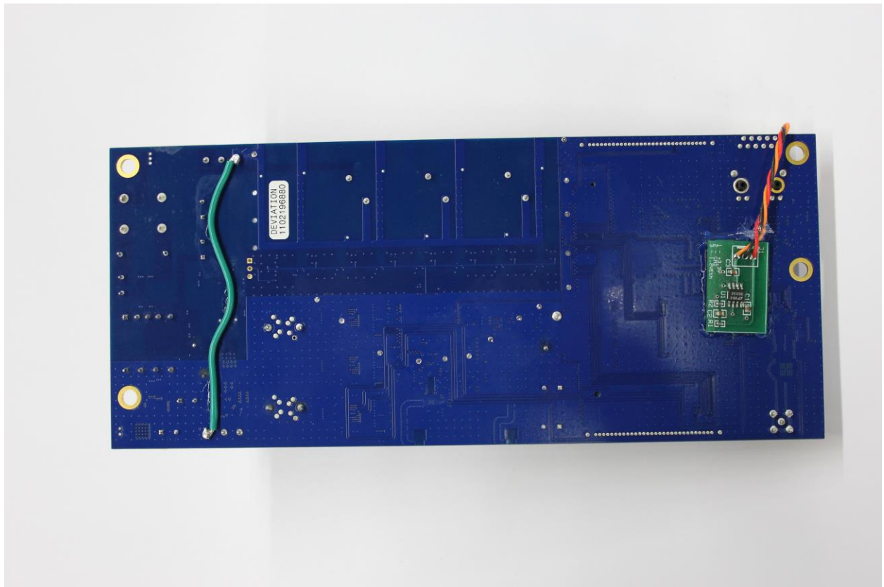
Photograph 7. Transformer Meter – Board Un-shielded - Back
