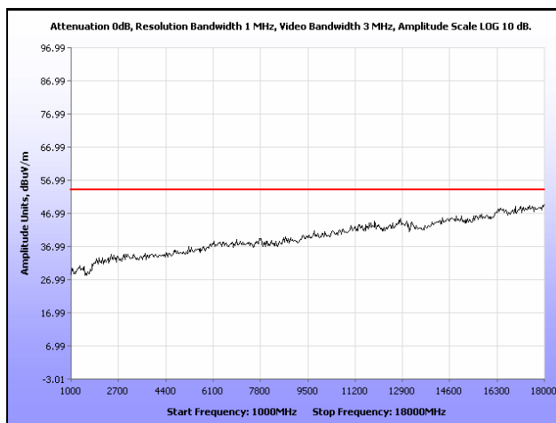
Plot 42. Radiated Spurious Emissions, High Channel, 802.11g, 1 GHz – 18 GHz, Peak under Average
