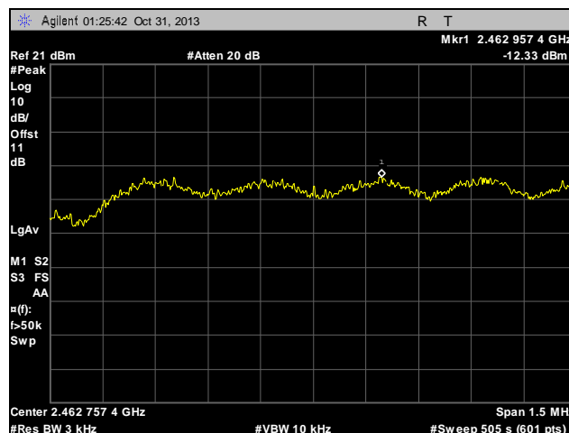
Plot 81. Peak Power Spectral Density, High Channel, 802.11n
