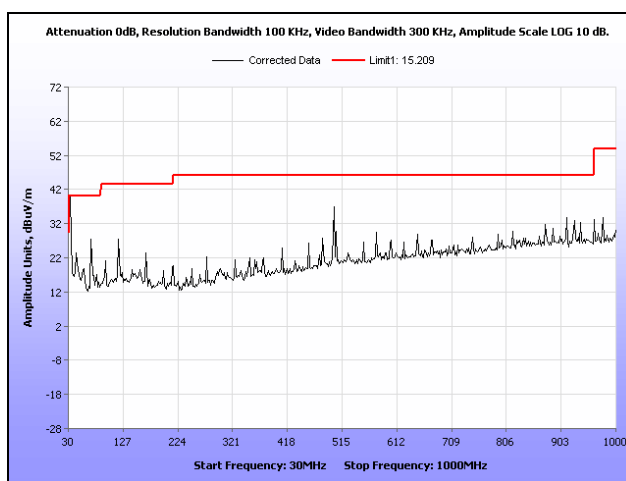
Plot 41. Radiated Spurious Emissions, High Channel, 802.11g, 30 MHz – 1 GHz
