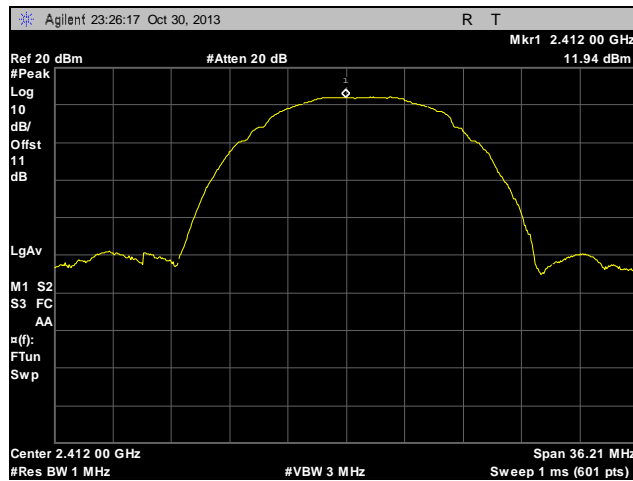
Plot 64. Peak Power Spectral Density, Determination, Low Channel, 802.11b
