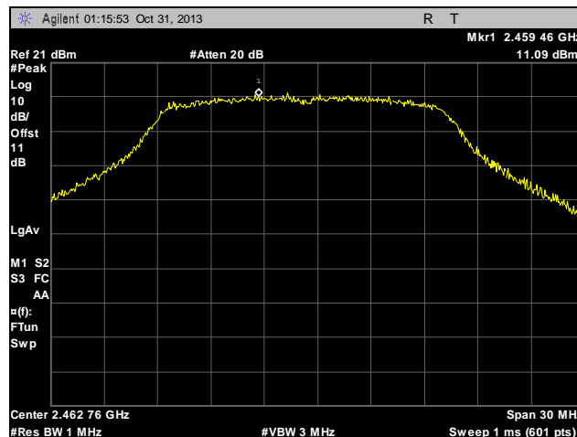
Plot 80. Peak Power Spectral Density, Determination, High Channel, 802.11n
