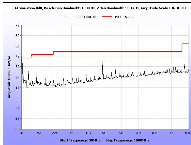
Plot 35. Radiated Spurious Emissions, High Channel, 802.11b, 30 MHz – 1 GHz
