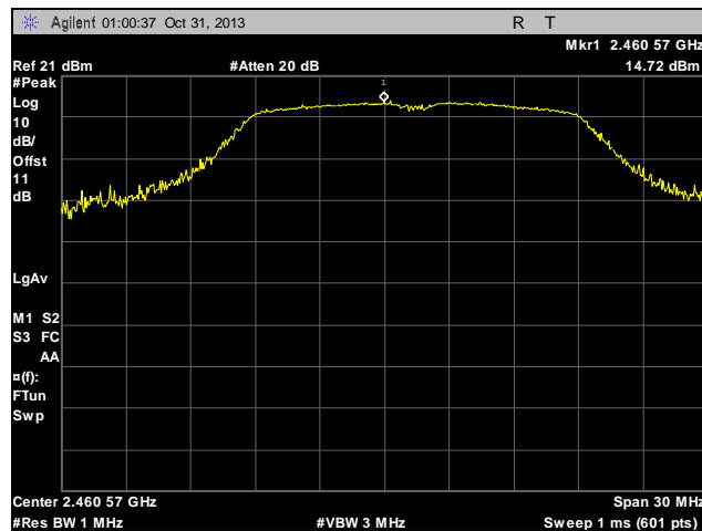
Plot 74. Peak Power Spectral Density, Determination, High Channel, 802.11g
