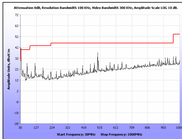
Plot 47. Radiated Spurious Emissions, High Channel, 802.11n, 30 MHz – 1 GHz
