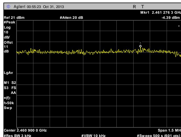
Plot 69. Peak Power Spectral Density, High Channel, 802.11b
