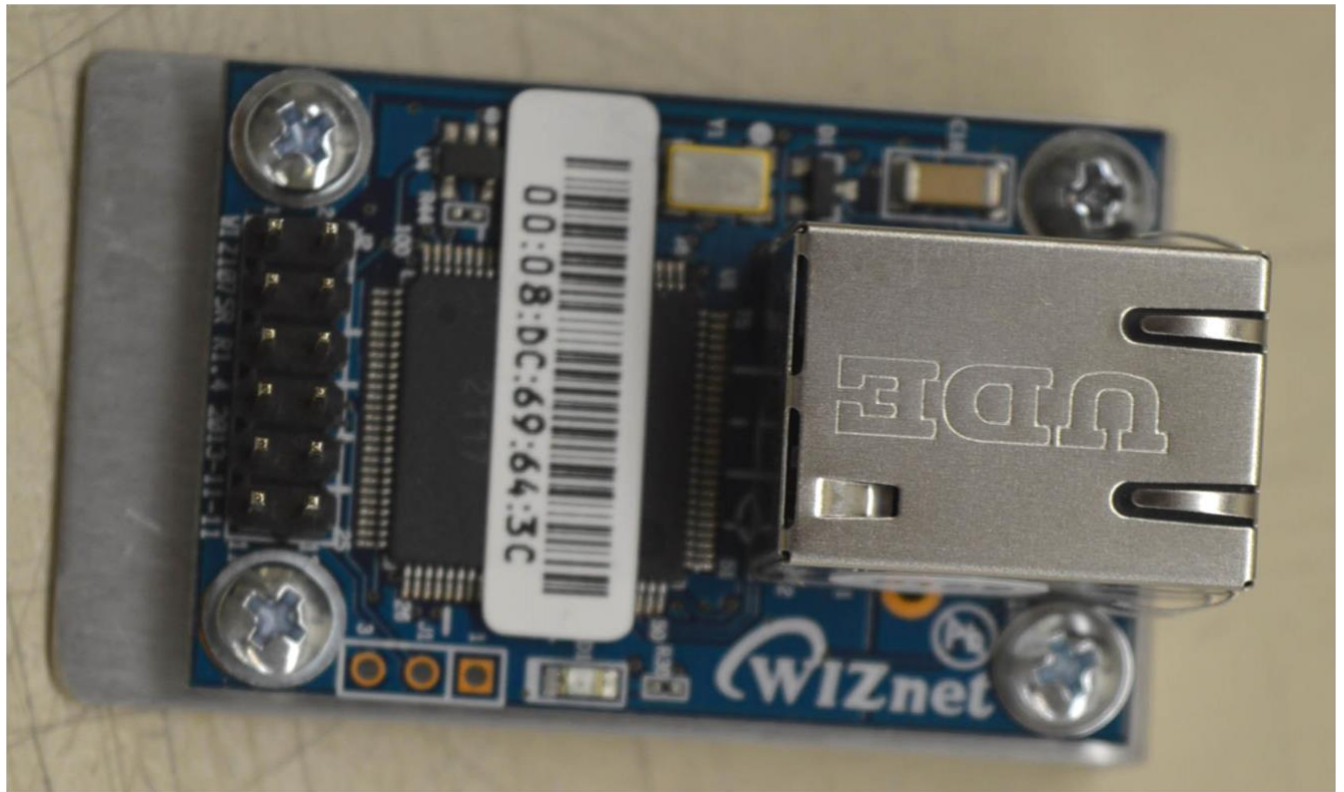
Ethernet Adapter – bottom
