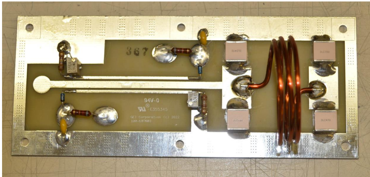
Filter & Coupler – Bottom
