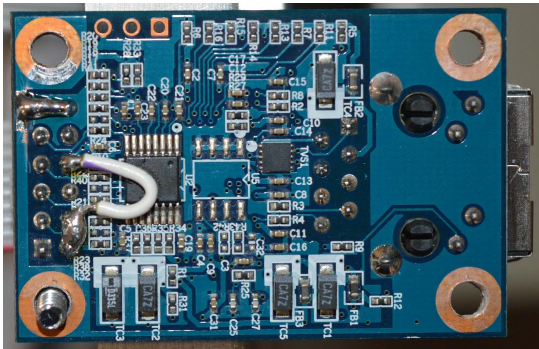
Ethernet Adapter – bottom
