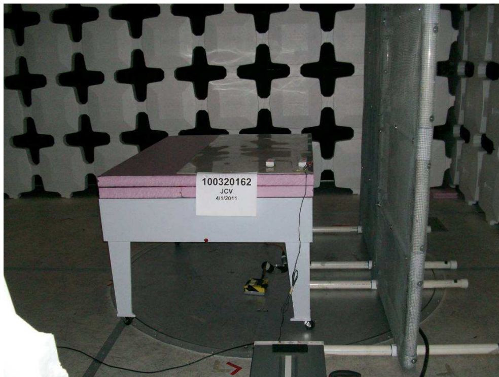
Side View
