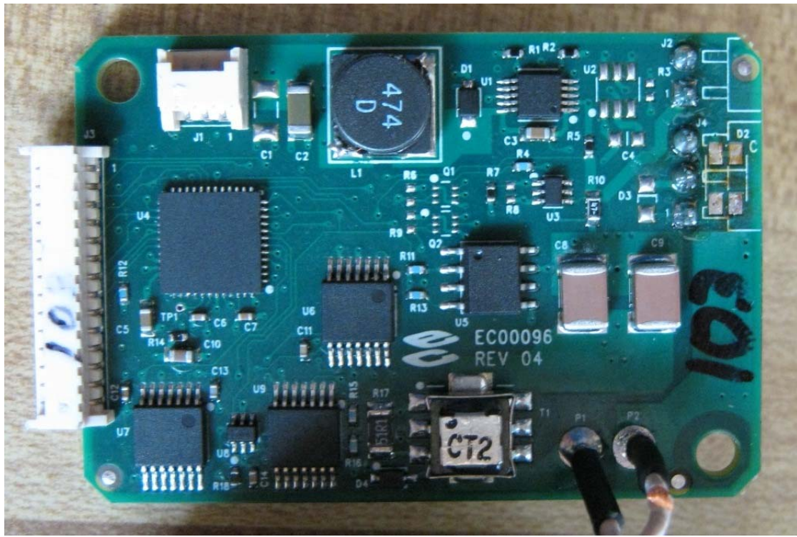
Photo Description: Circuit Board – Side 2
