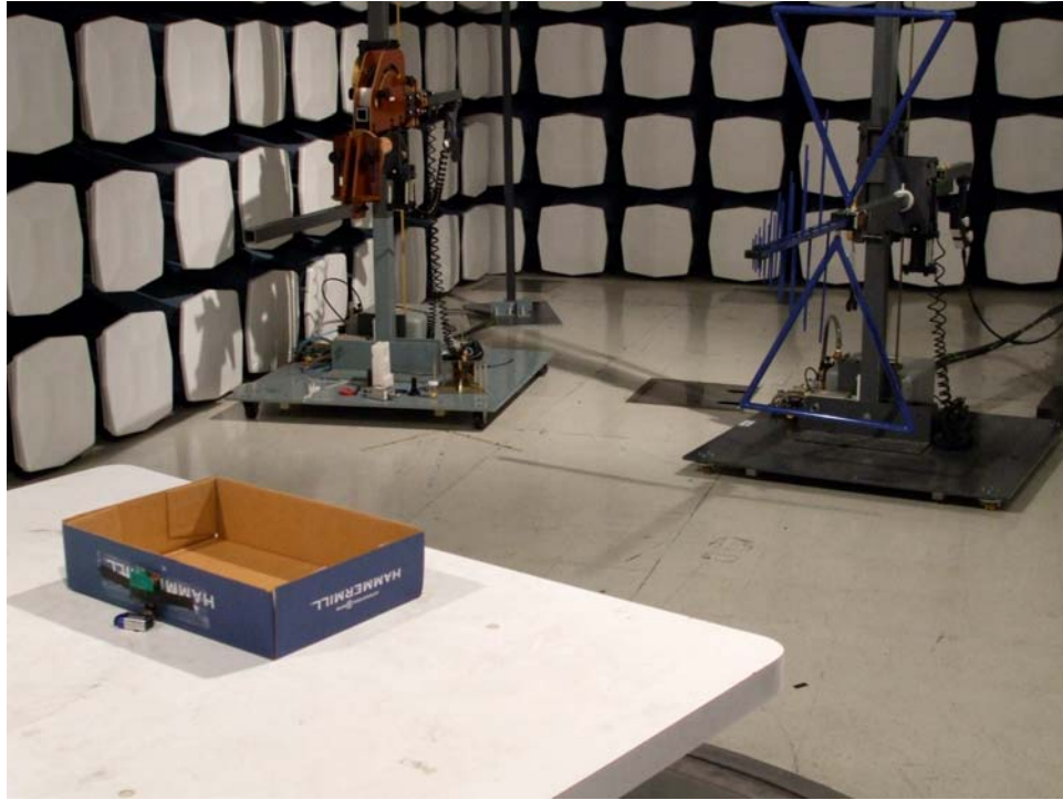
VIEW FROM THE TURNTABLE DURING 30-1000MHZ TEST 5m SEMIANECHOIC CHAMBER LEXMARK INTERNATIONAL, LEXINGTON KY
