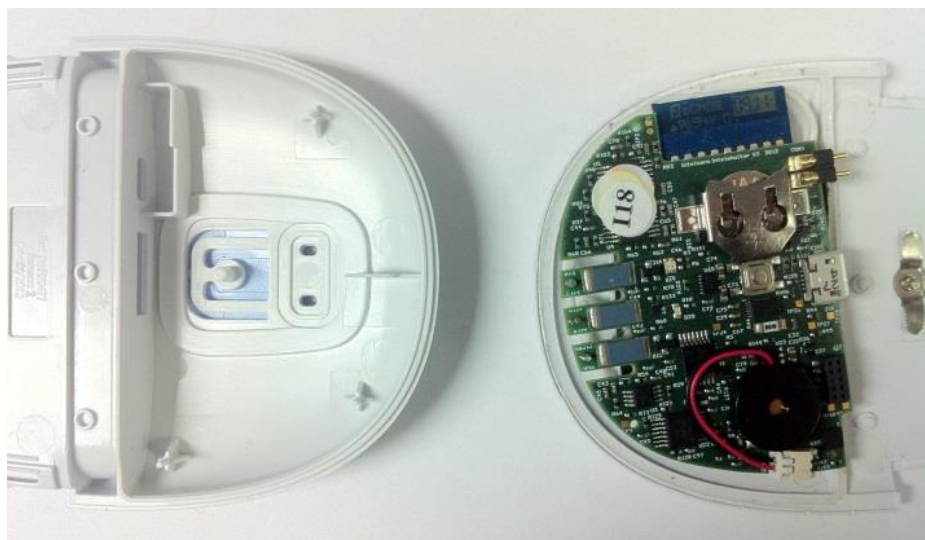
sensor Device View of inside top case and PCB underside
