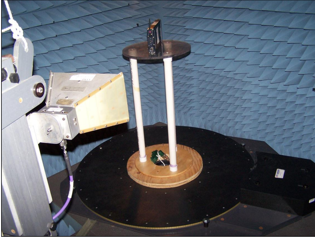
Photograph 3. Radiated Spurious Emissions, Test Setup – 2
