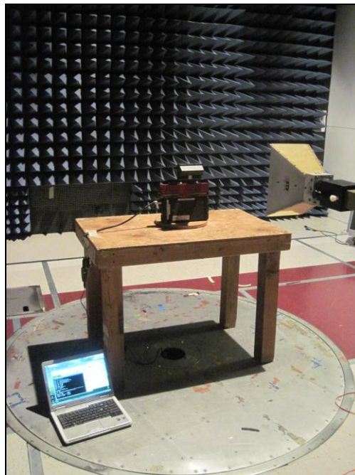
Photograph 3. Radiated Spurious Emissions 1 – 18 GHz Test Setup
