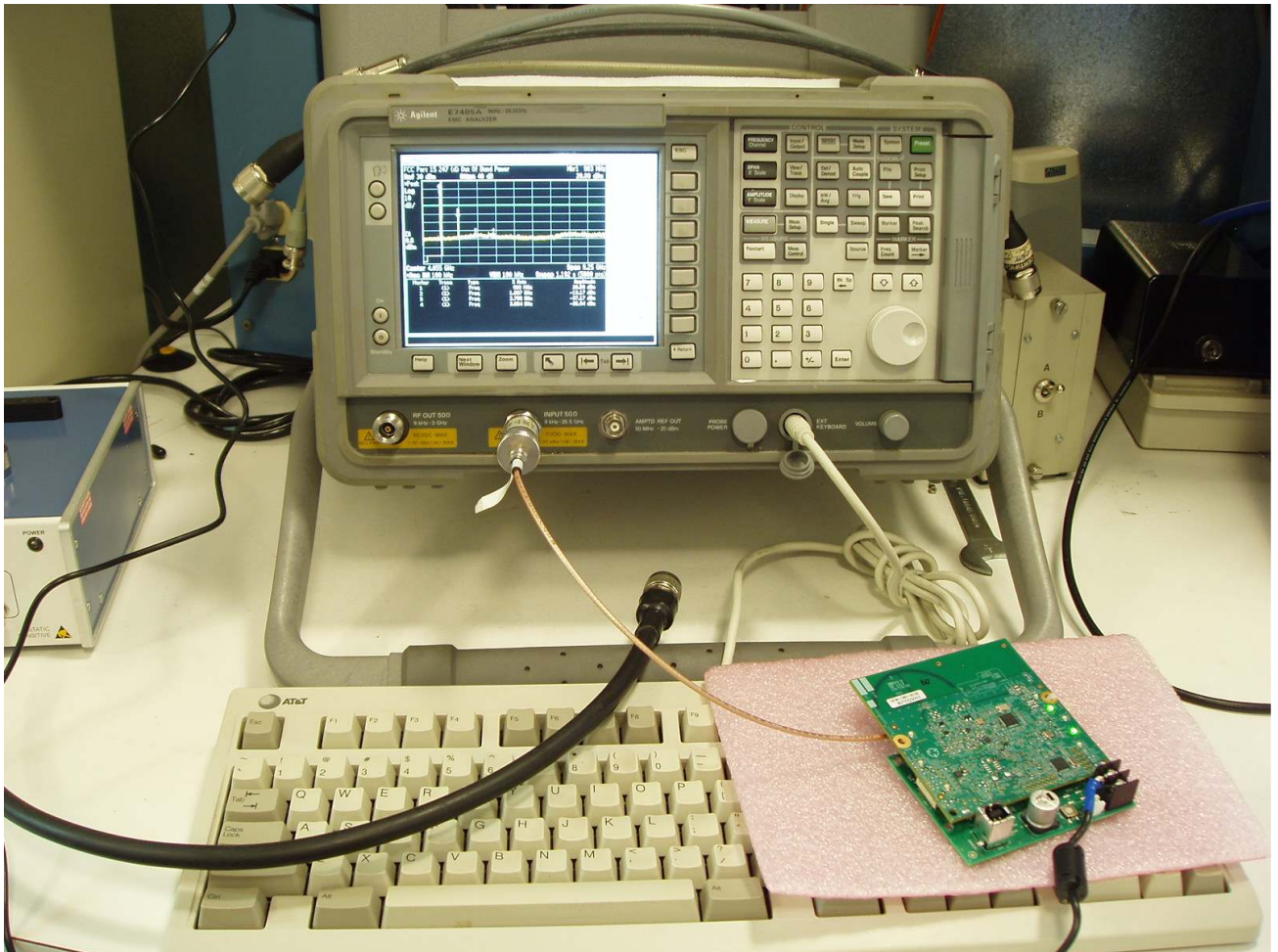
Photo 5 – Antenna Port Conducted Test Set-up
