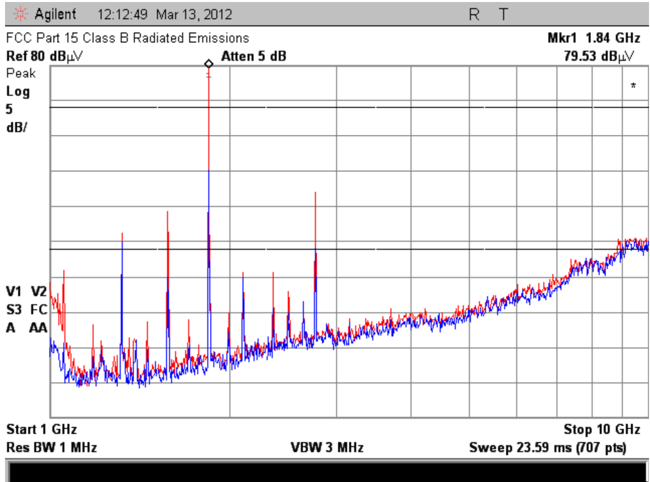
Figure 5.2-15 – Radiated Emissions 1 – 10 GHz (Peak Detector) Channel 49
