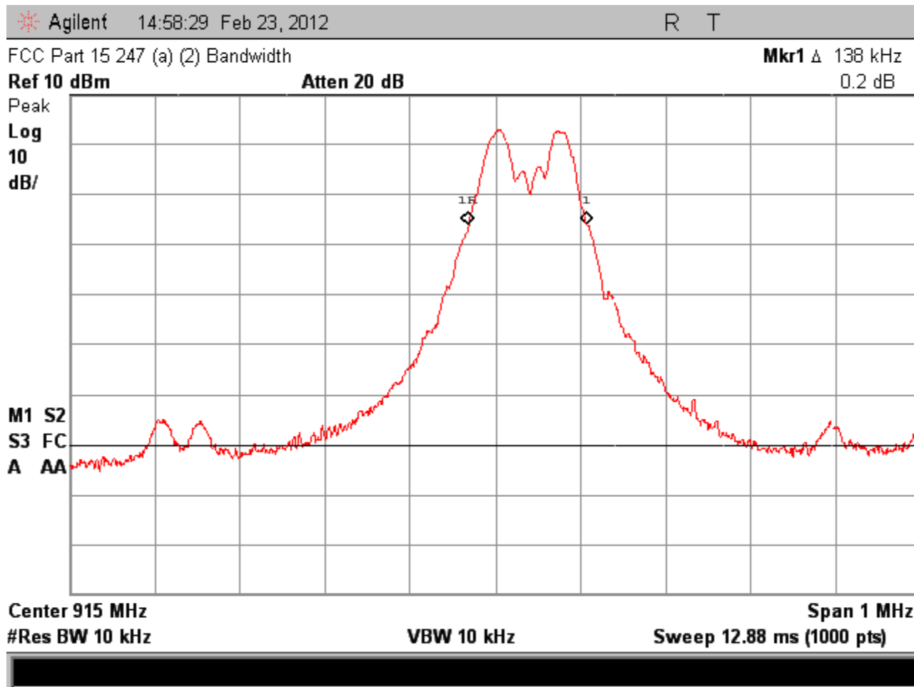
Figure 7.2-2 – Channel 24 Bandwidth
