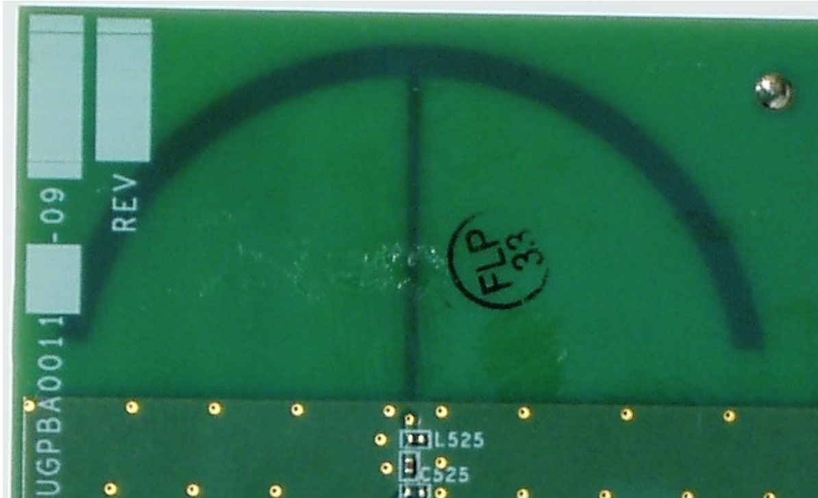
Photo 6.3-1 – Internal Antenna
