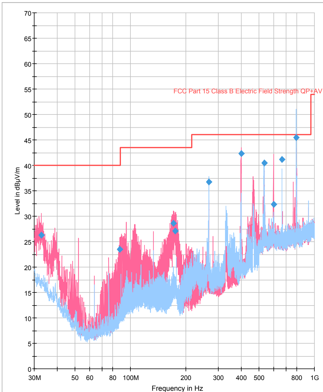
Figure 5.2-5 – Final Radiated Emissions Plot for the 30 – 1000 MHz Band
