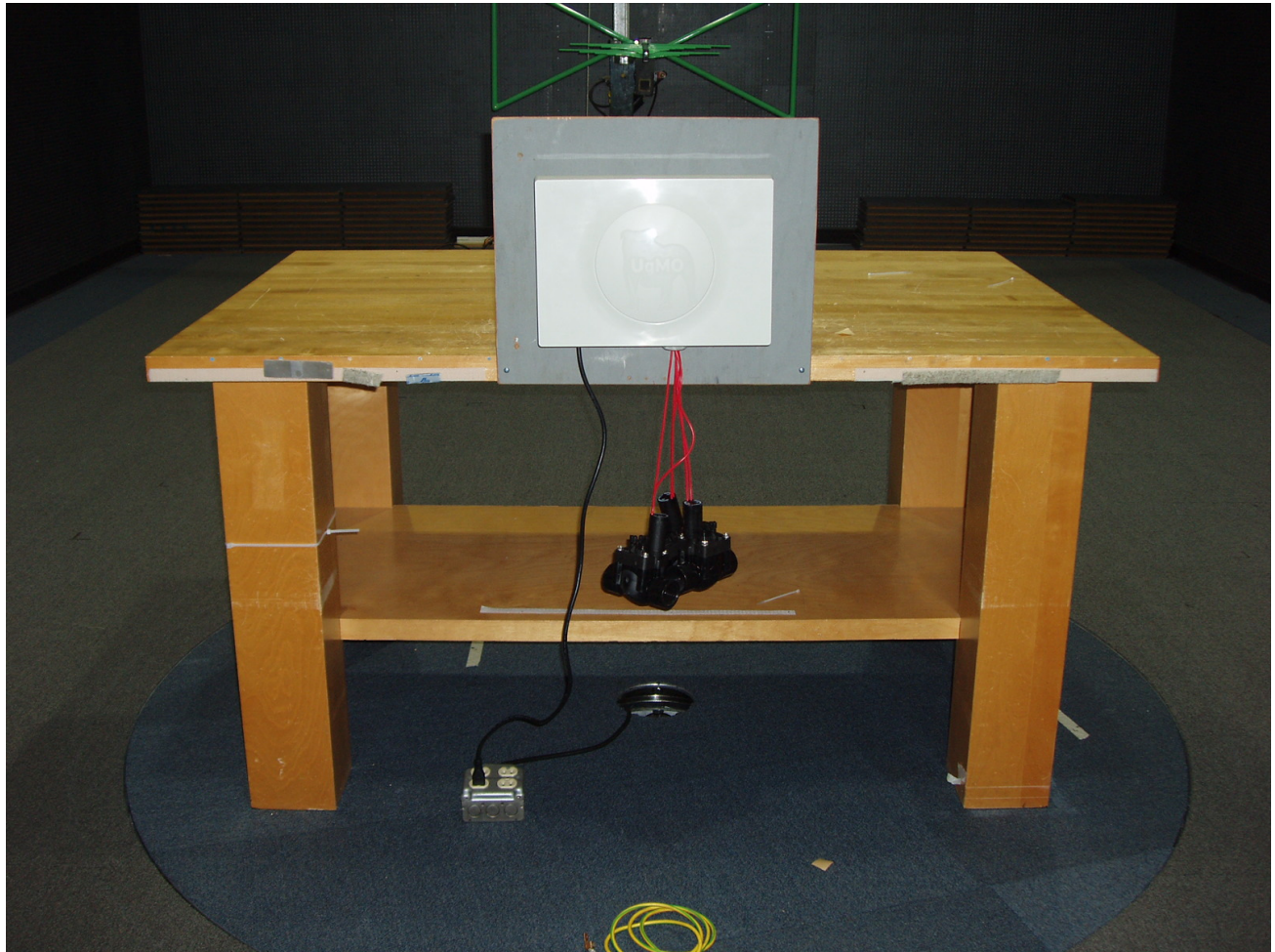
Photo 5.5-2 - Rear View of the Radiated Emissions Test Set-up
