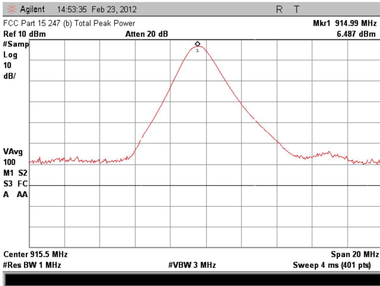
Figure 8.2-2 – Channel 24 Signal Power
