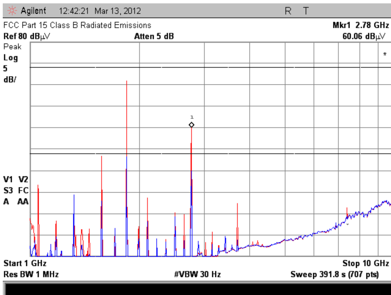
Figure 5.2-16 – Radiated Emissions 1 – 10 GHz (Average Detector) Channel 49
