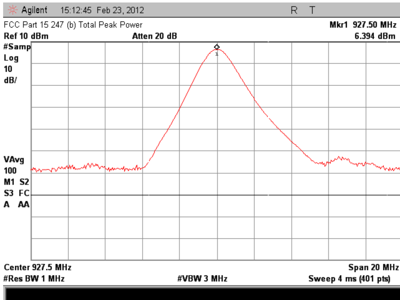
Figure 8.2-3 – Channel 49 Signal Power
