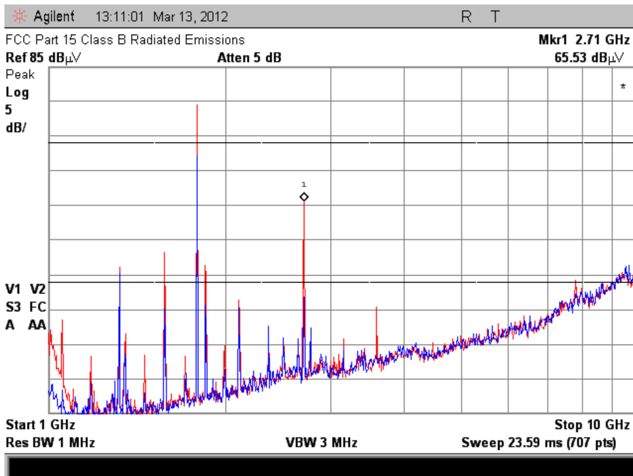
Figure 5.2-12 – Radiated Emissions 1 – 10 GHz (Peak Detector) Channel 0
