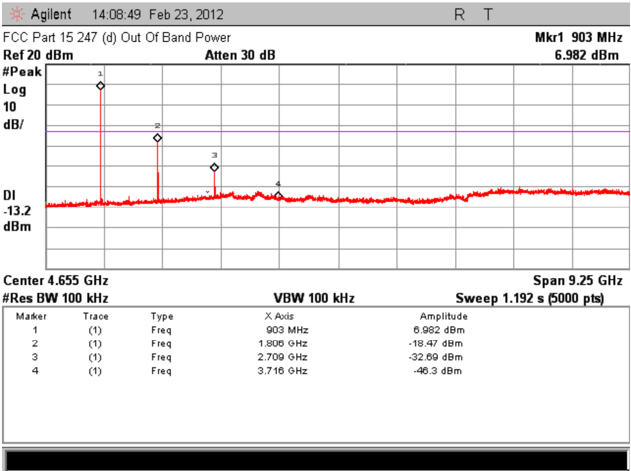
Figure 9.2-1 – Out of Band Conducted Data for Channel 0
