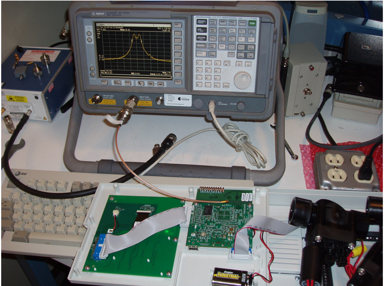
Photo 3 – Antenna Port Conducted Test Set-up
