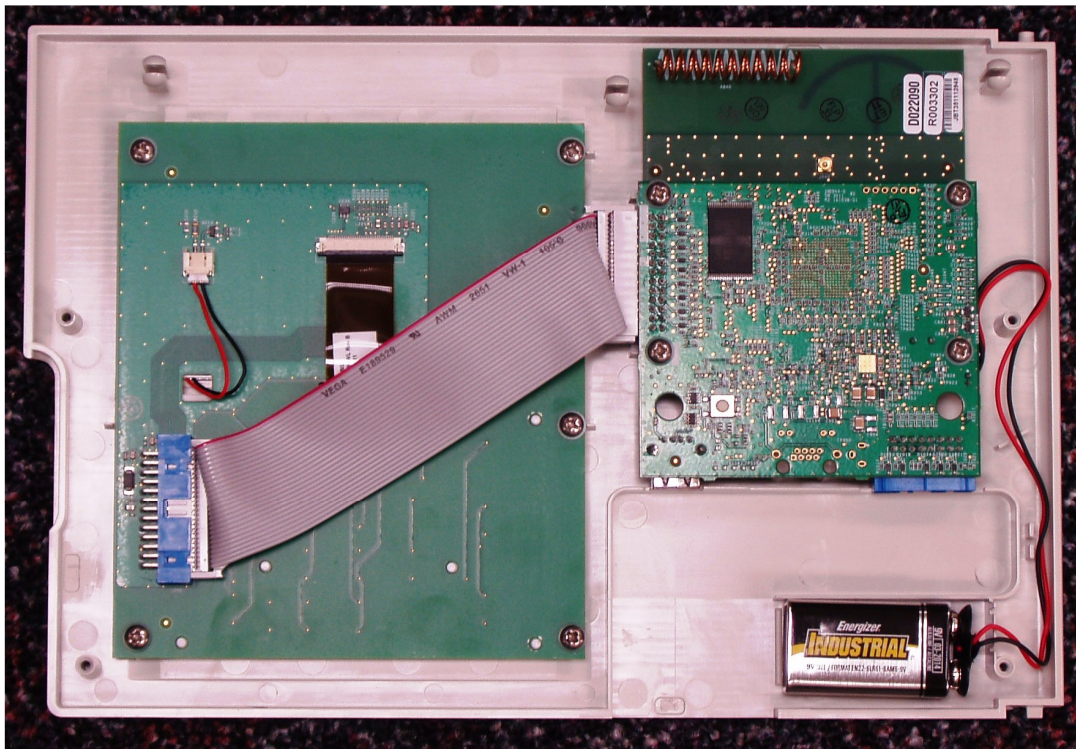
Photo 5 – Boards Mounted in the Enclosure
