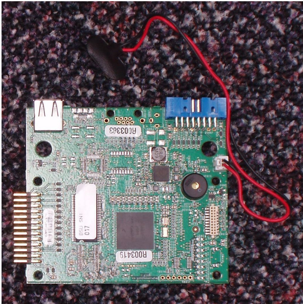
Photo 3 – Top View of the Main Board
