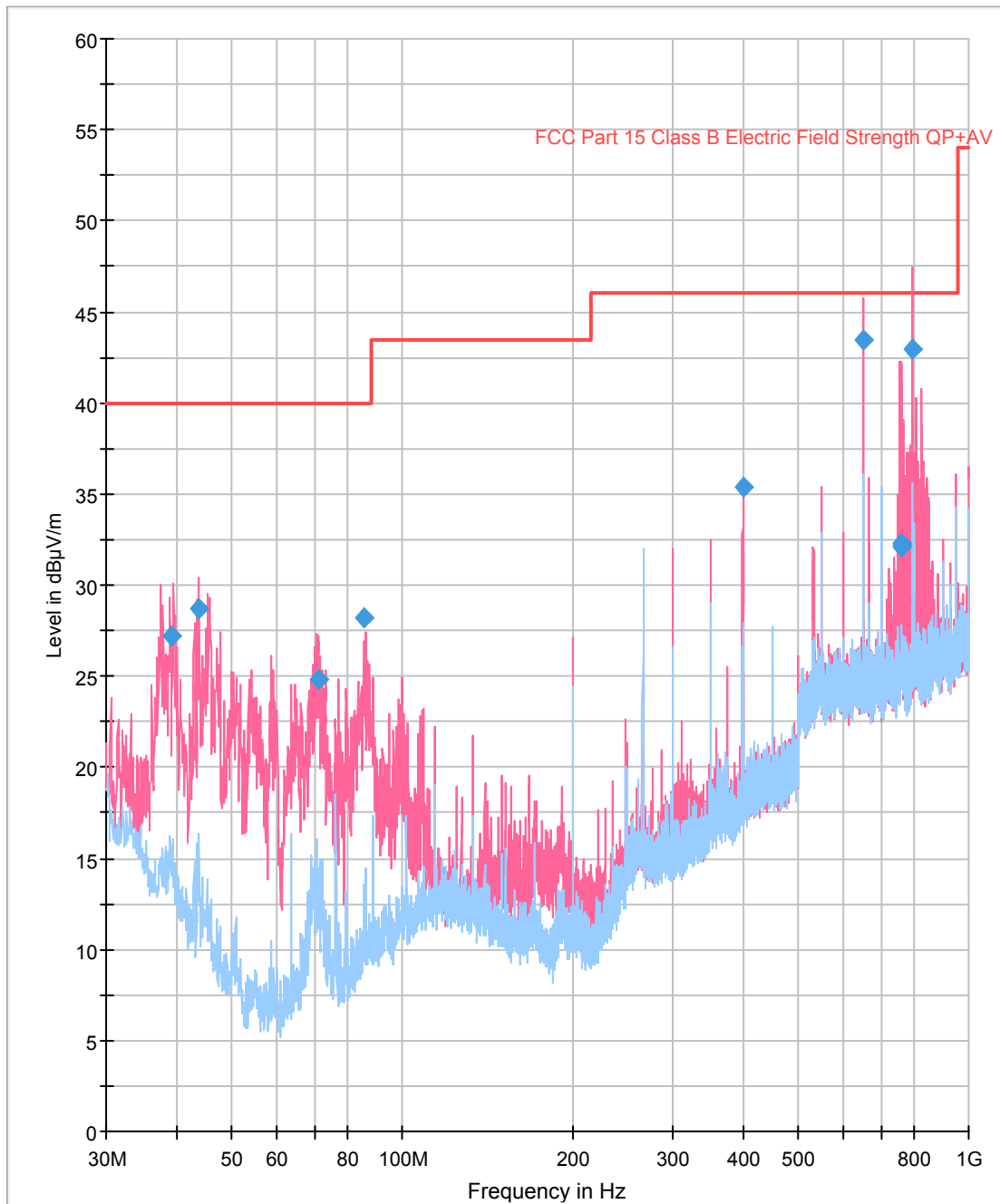
Figure 5.2-1 – FCC Part 15 Class B Radiated Emissions Plot
