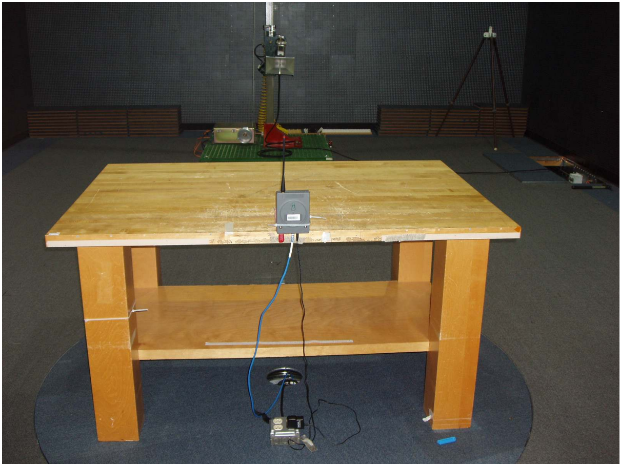
Photo 5.5-3 - Rear View of the Radiated Emissions Test Set-up above 1 GHz
