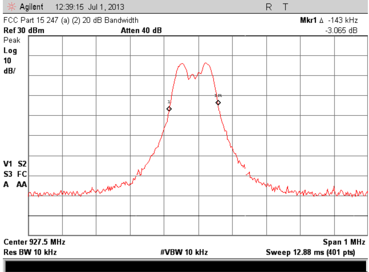
Figure 7.2-3 – Channel 49 Bandwidth
