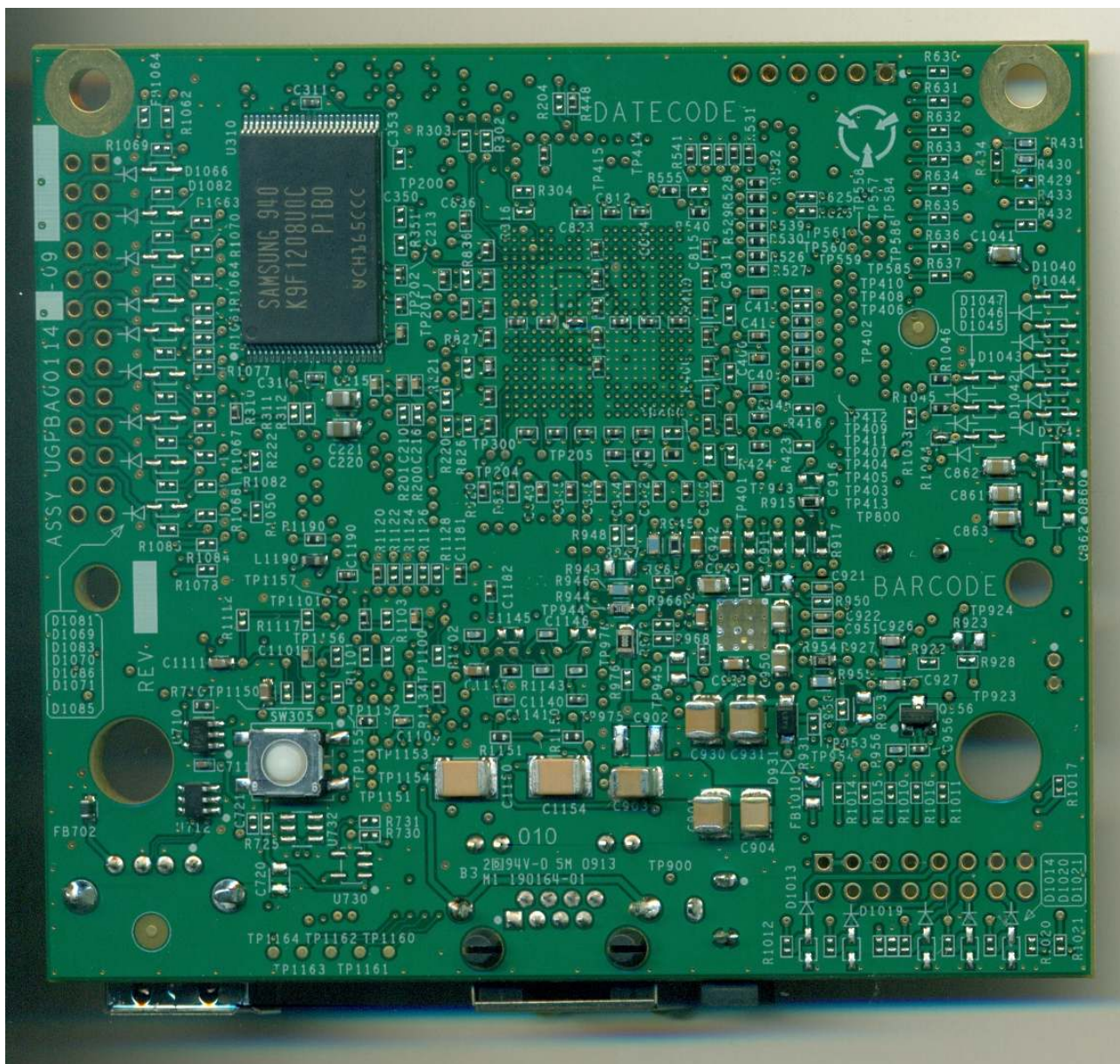
Photo 4 – Bottom Top View of the Main Board
