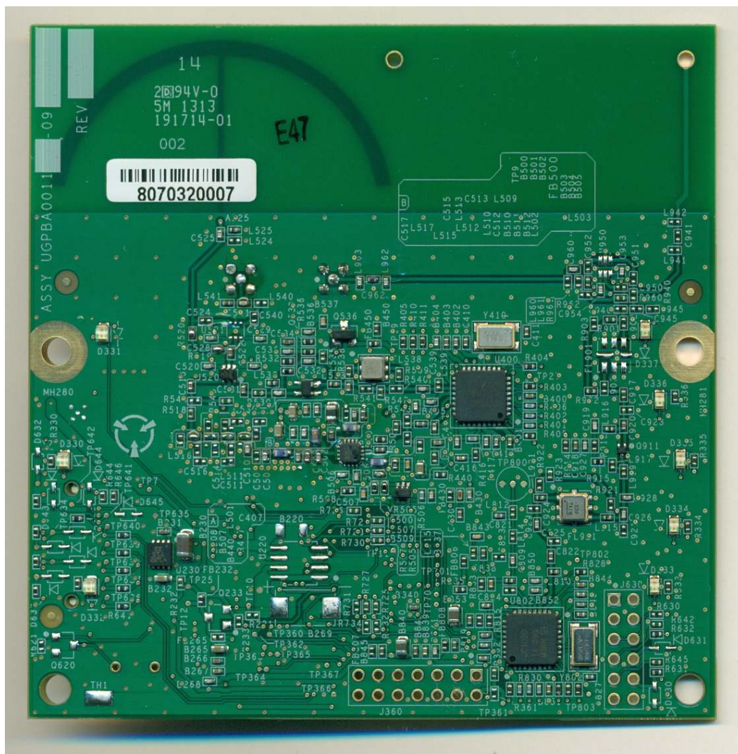
Photo 1 – Top View of the Radio Board
