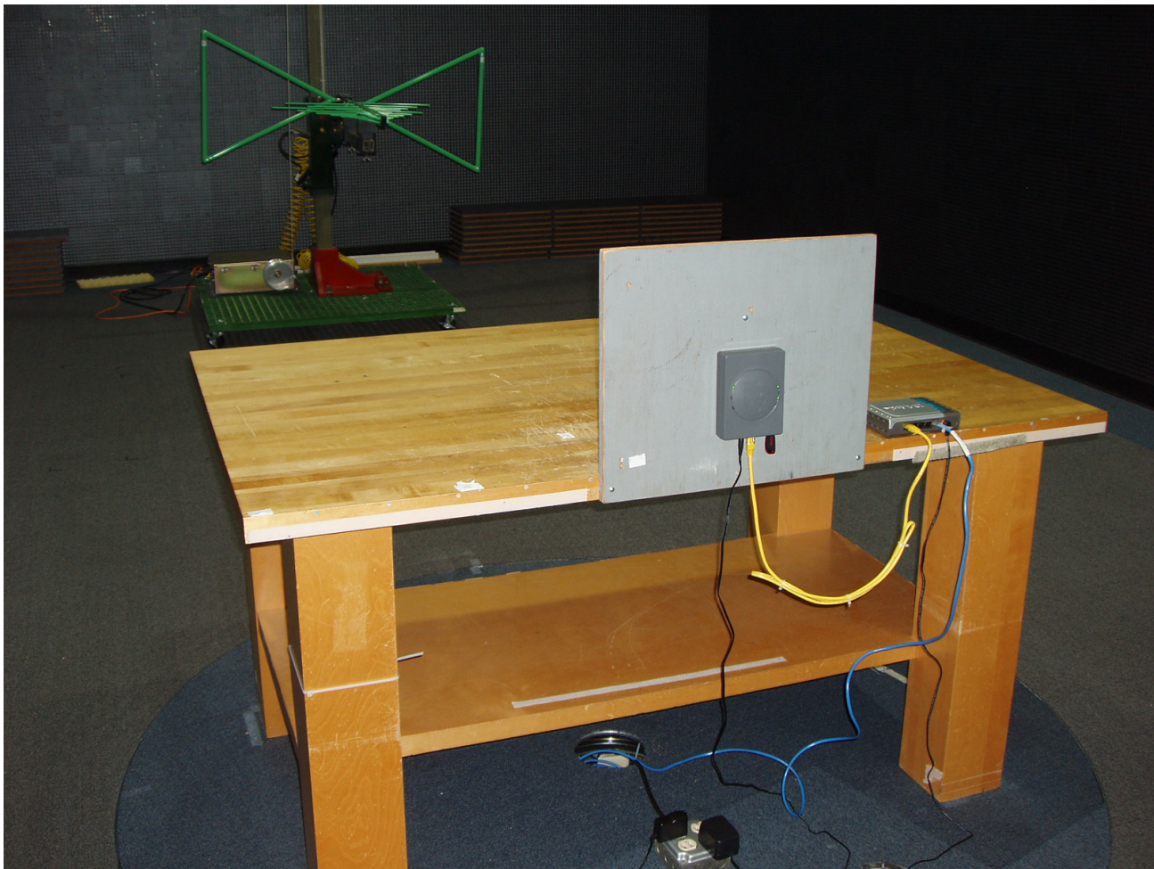
Photo 2 – Rear View of the Radiated Emissions Test Set-up
