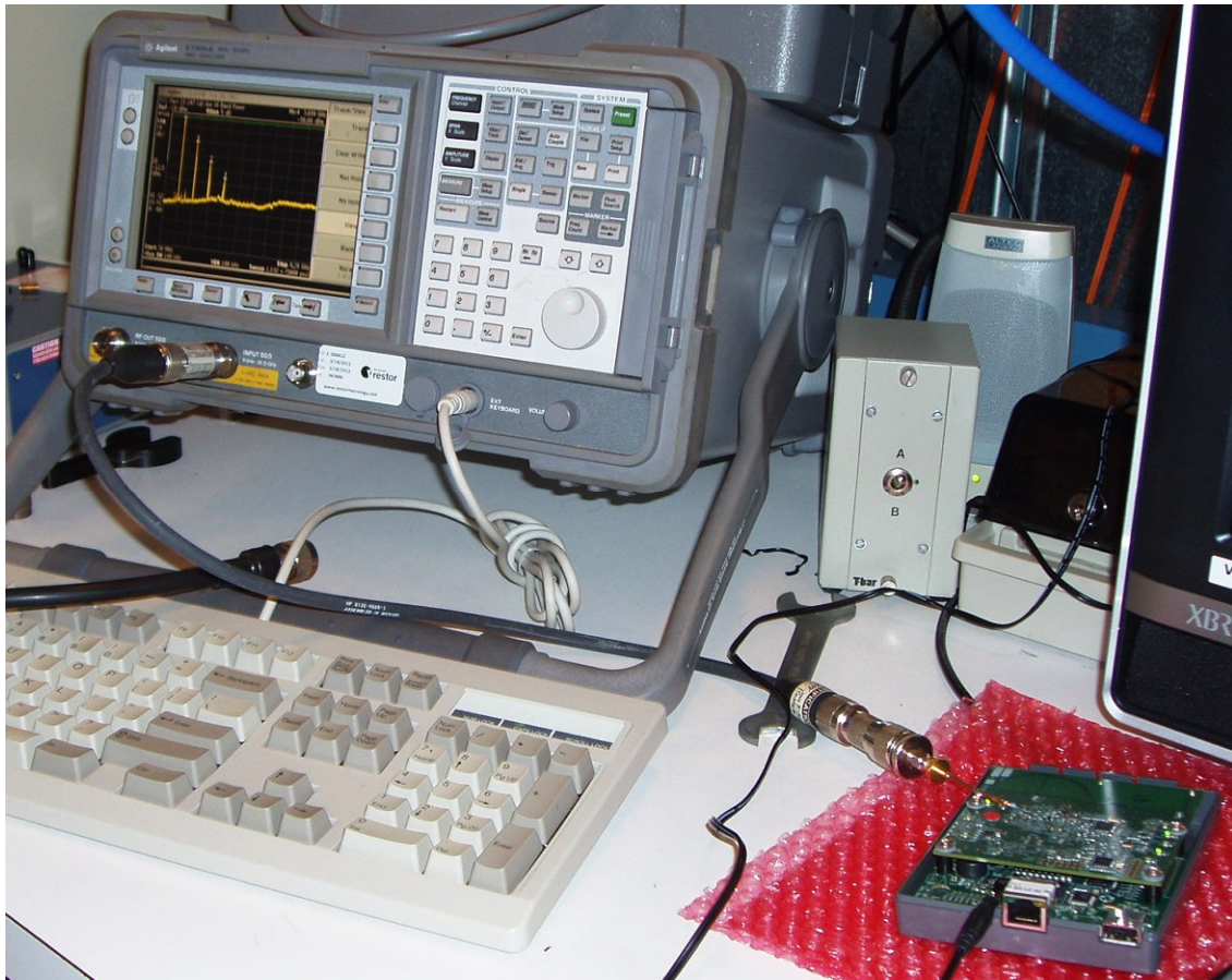
Photo 4 – Antenna Port Conducted Test Set-up
