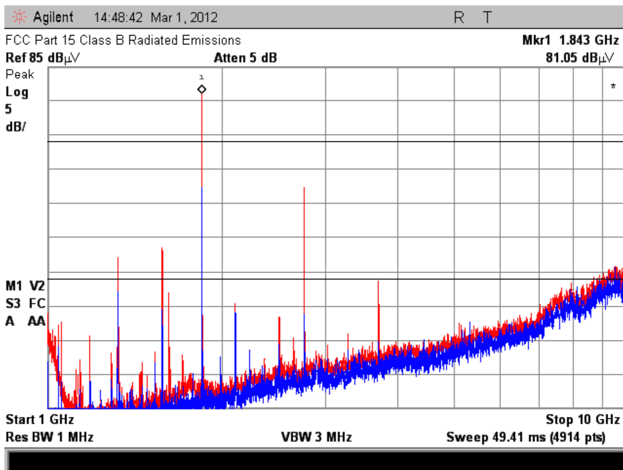
Figure 5.2-13 – Radiated Emissions 1 – 10 GHz (Peak Detector) Channel 49
