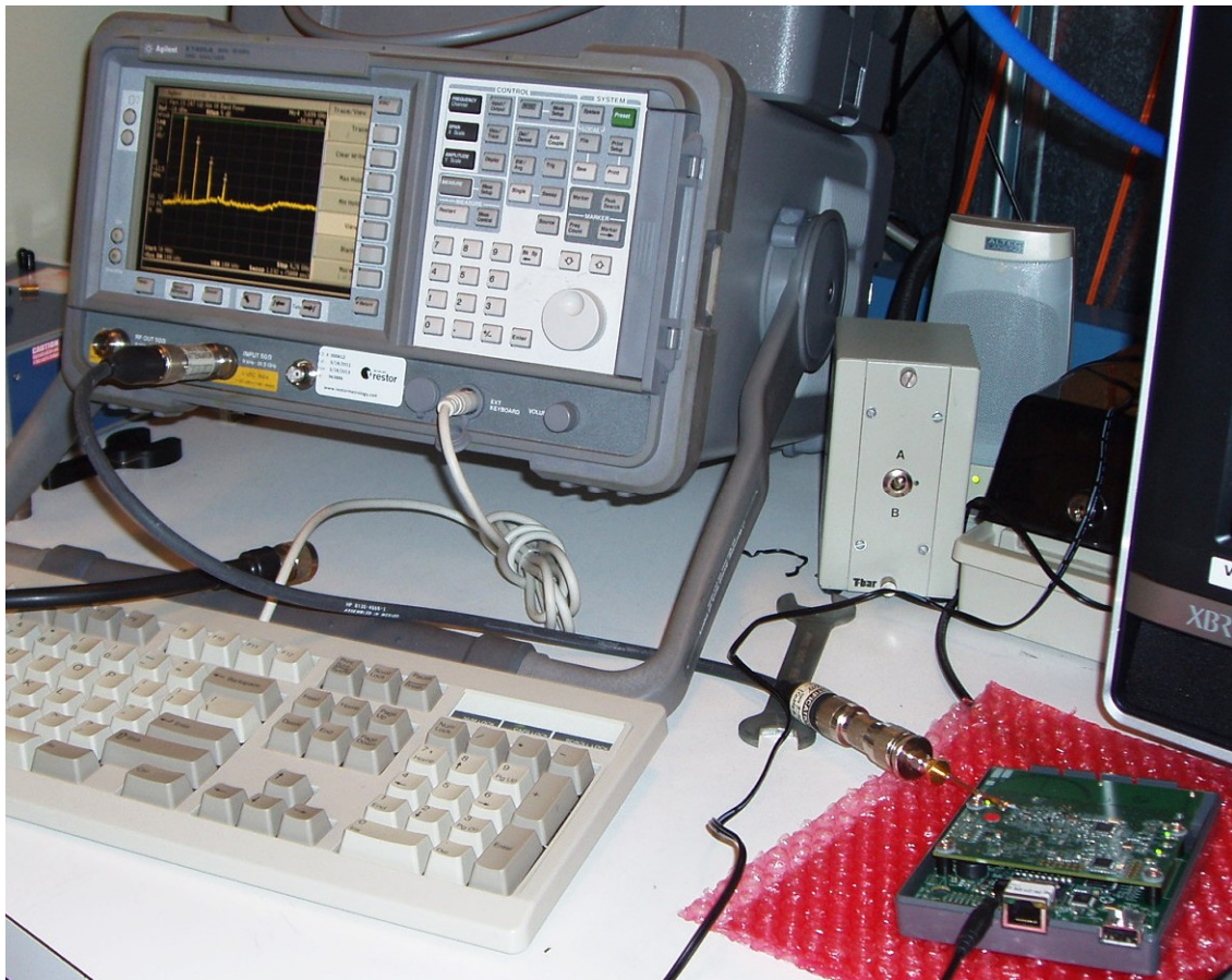
Photo 7.4-1 – Conducted Measurement Test -Setup
