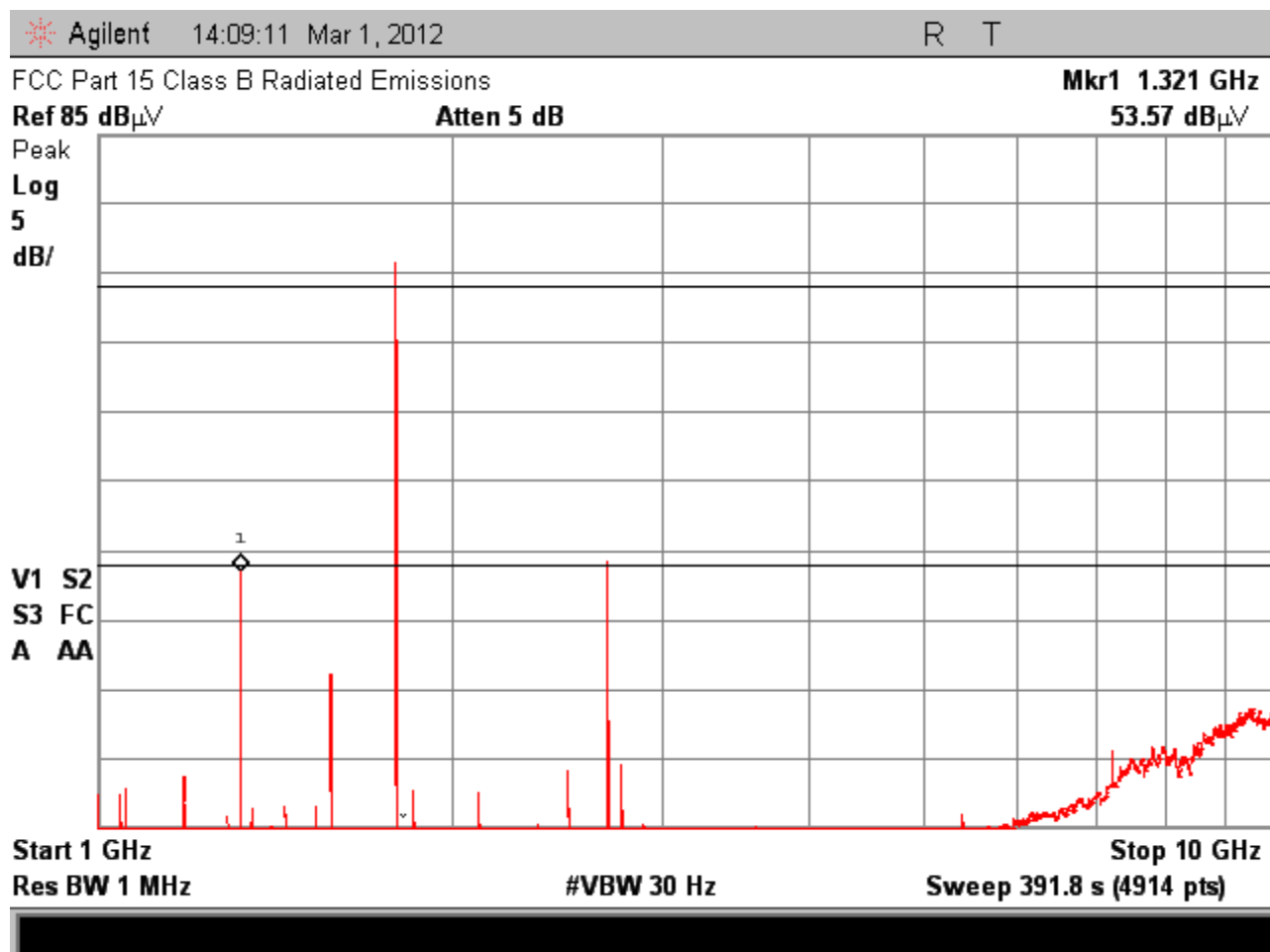
Figure 5.2-11 – Radiated Emissions 1 – 10 GHz (Average Detector) Channel 0
