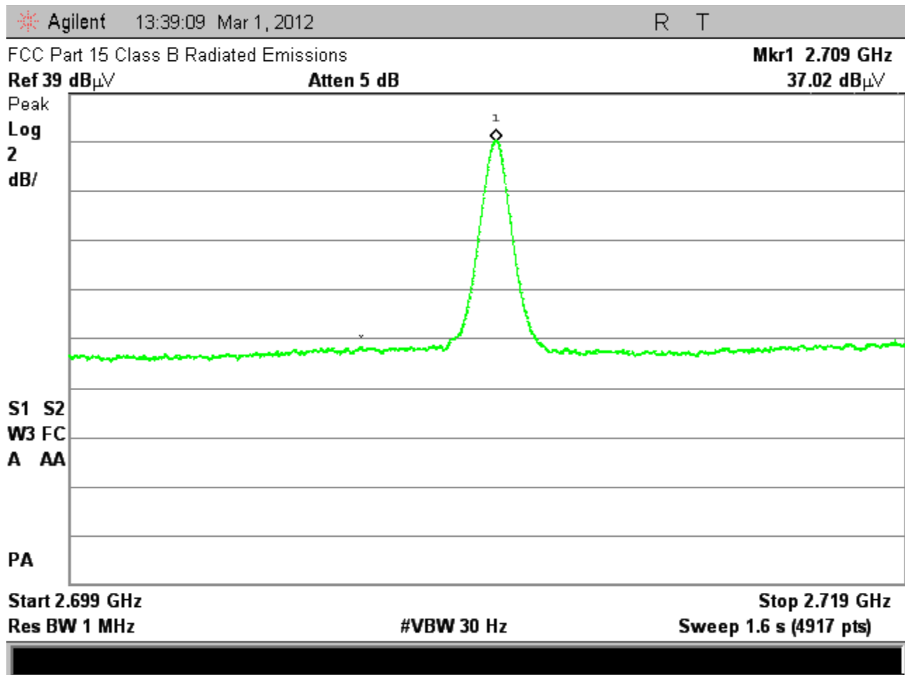
Figure 5.2-12 – Zoomed Average Field Strength Measurement of the Third Harmonic for Channel 0 Operation
