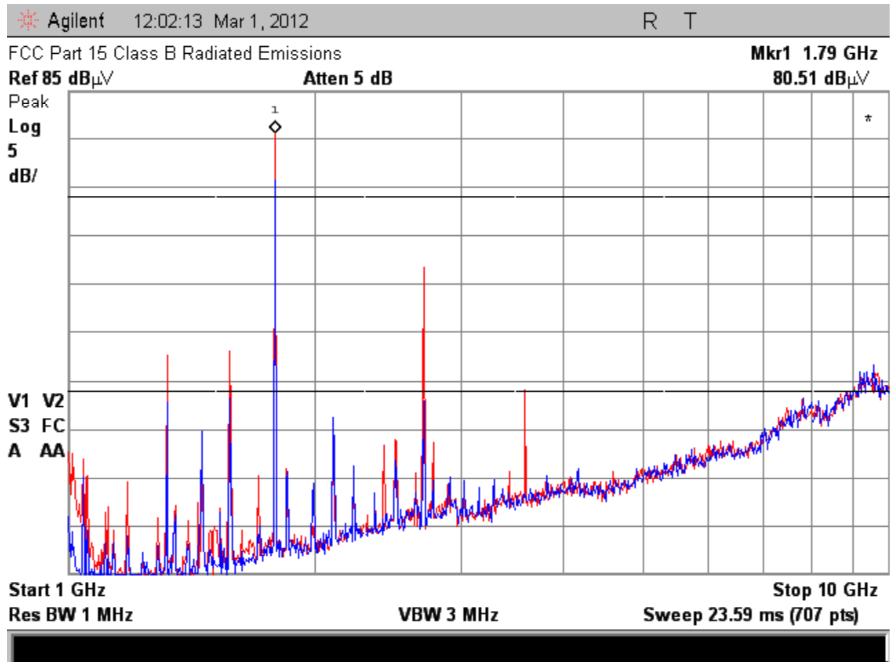
Figure 5.2-10 – Radiated Emissions 1 – 10 GHz (Peak Detector) Channel 0
