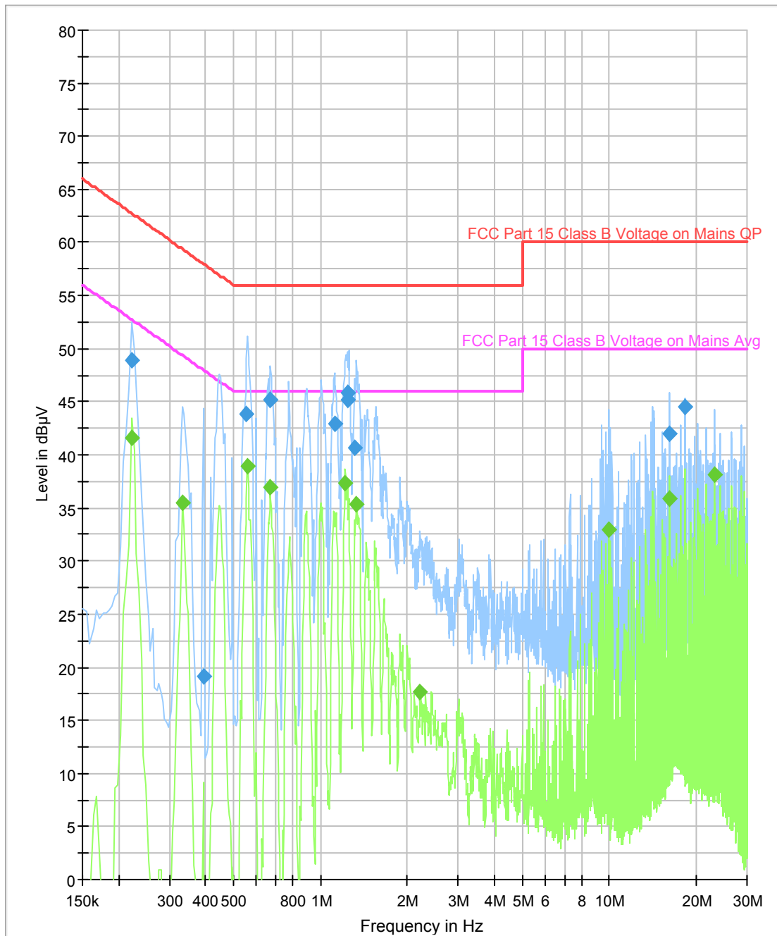
Figure 4.2-1 – FCC Part 15 Class B Conducted Emissions Plot
