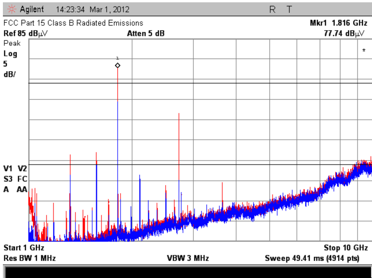
Figure 5.2-9 – Radiated Emissions 1 – 10 GHz (Peak Detector) Channel 24
