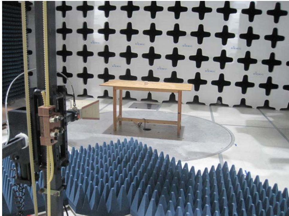
Radiated Emission (>1GHz) Setup Front View
