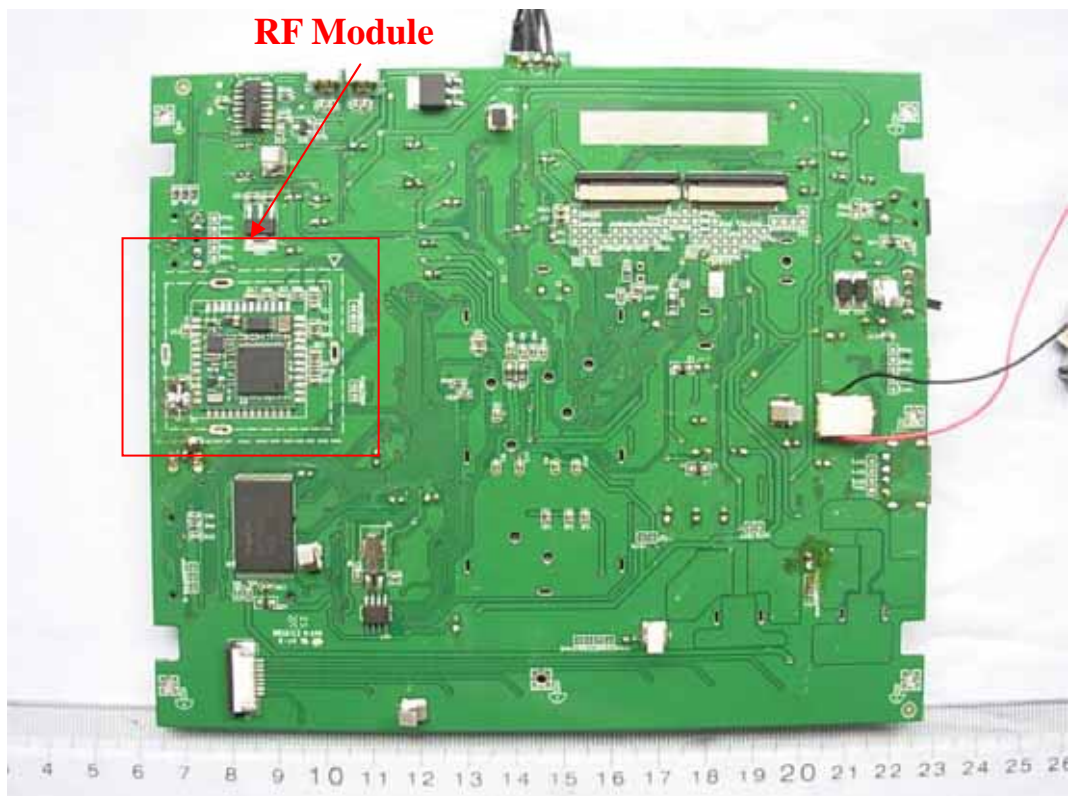
FIGURE 7 10.1 INCH DIGITAL PHOTO FRAME (M/N: LP-101WT) MAIN BOARD (SOLDERED SIDE)
