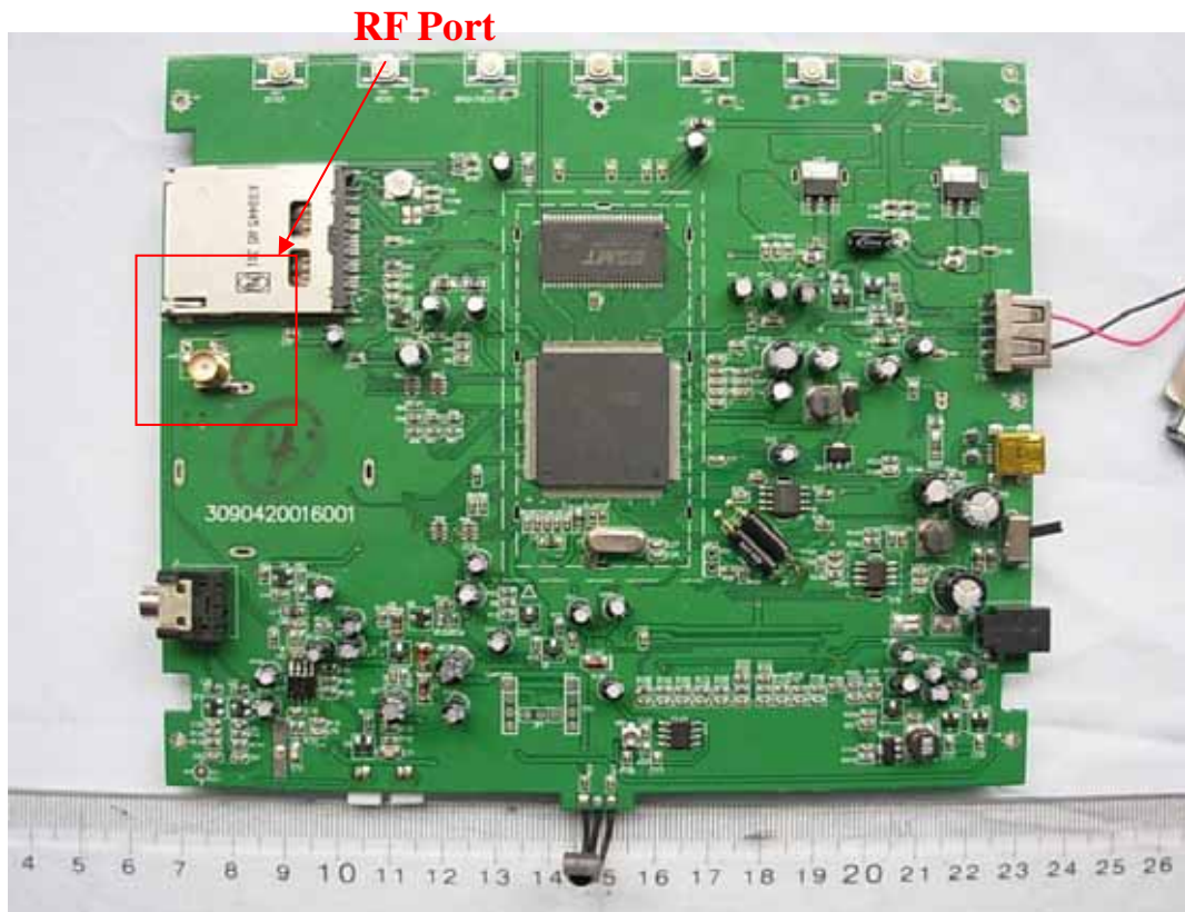
FIGURE 6 10.1 INCH DIGITAL PHOTO FRAME (M/N: LP-101WT) MAIN BOARD (COMPONENT SIDE)
