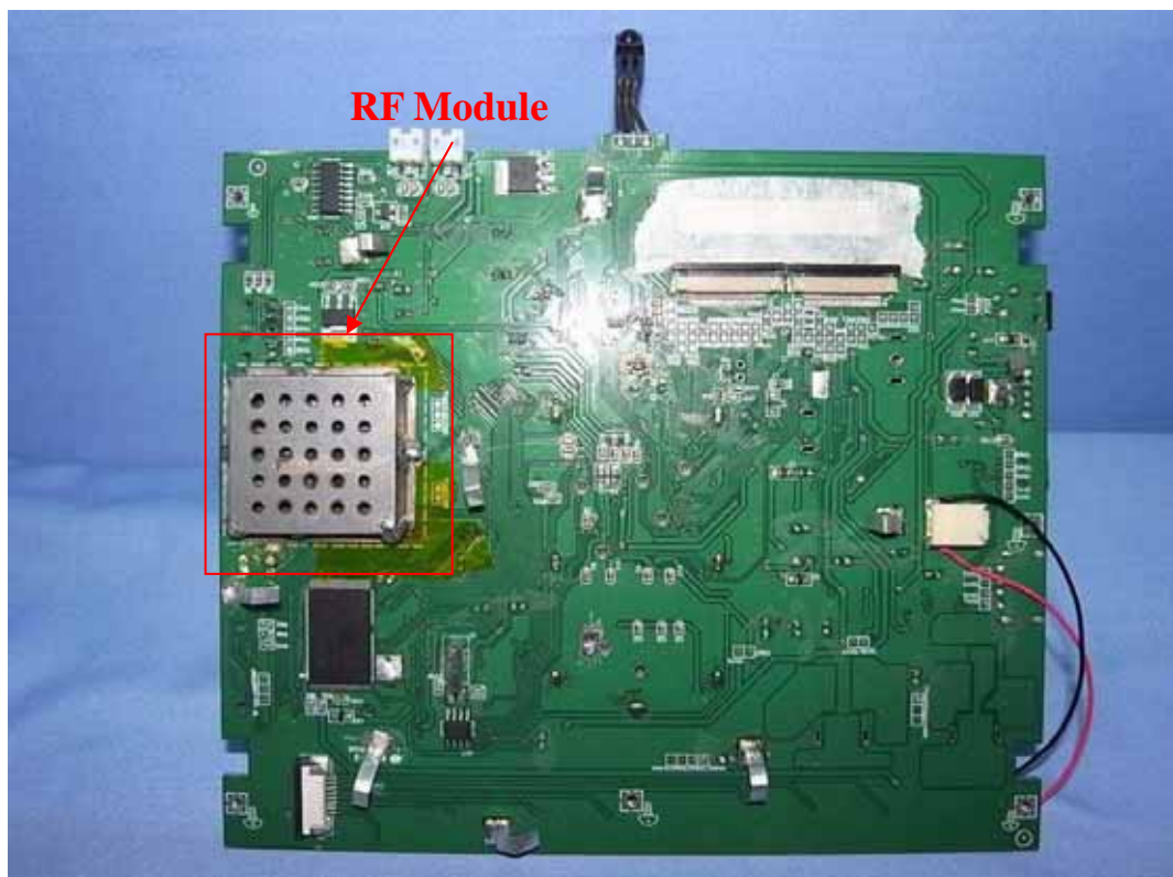
FIGURE 5 10.1 INCH DIGITAL PHOTO FRAME (M/N: LP-101WT) MAIN BOARD BACK SHIELDED
