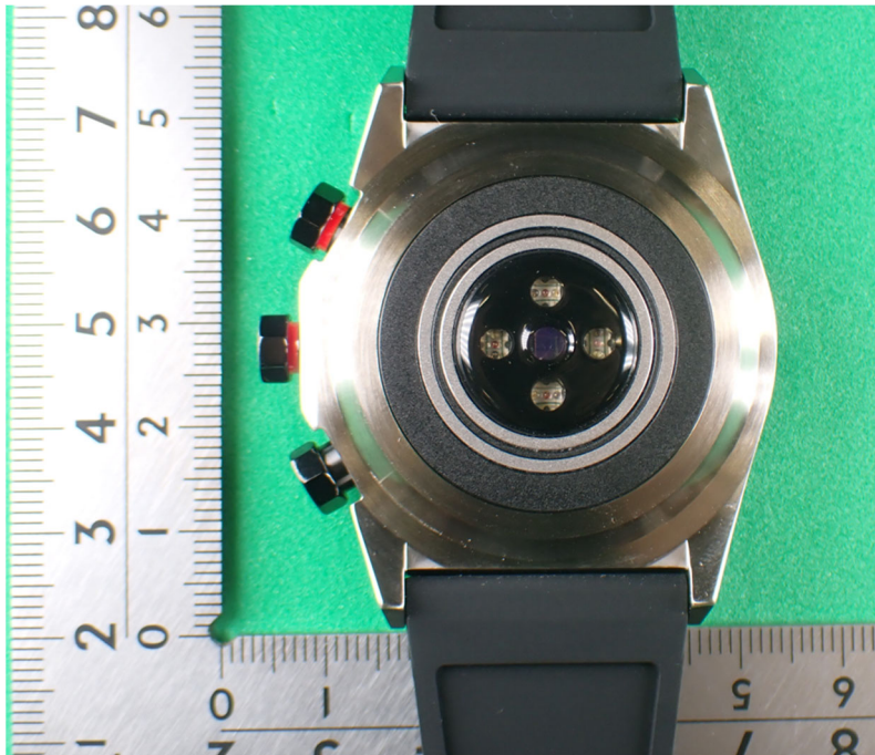
Back side
