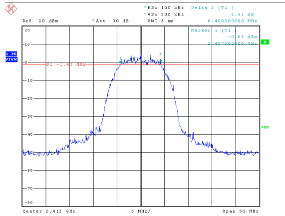
Modulation Type: 802.11b, ANT 0 CH01
