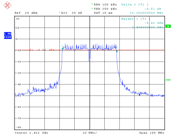
Modulation Type: 802.11n HT40, ANT 0 CH03
