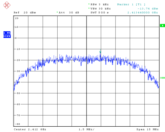
Modulation Type: 802.11b, ANT 0 CH01
