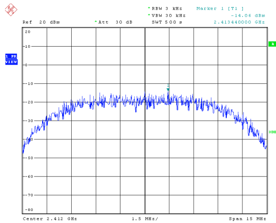
Modulation Type: 802.11b, ANT 1 CH01
