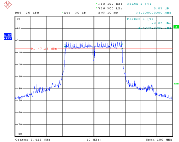
Modulation Type: 802.11n HT40, ANT 1 CH03
