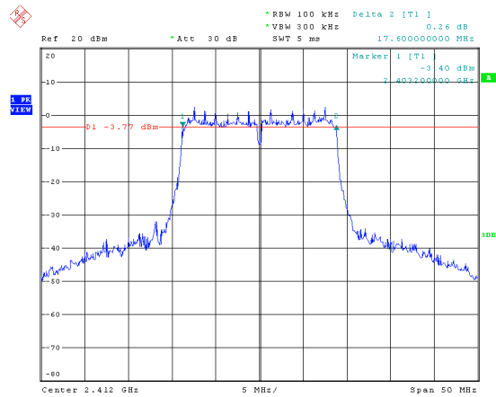
Modulation Type: 802.11n HT20, ANT 1 CH01
