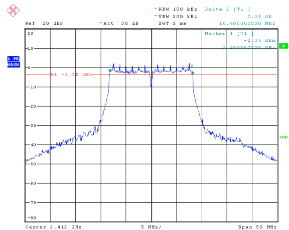
Modulation Type: 802.11g, ANT 1 CH01
