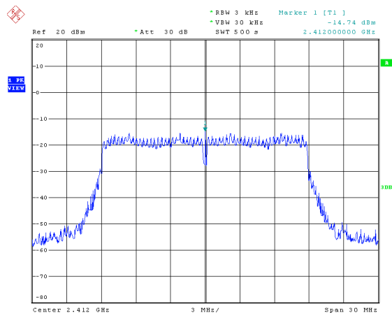
Modulation Type: 802.11n HT20, ANT 1 CH01
