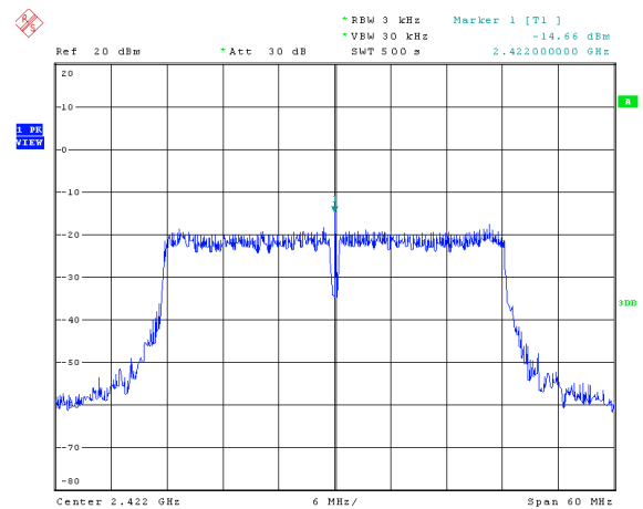
Modulation Type: 802.11n HT40, ANT 1 CH03
