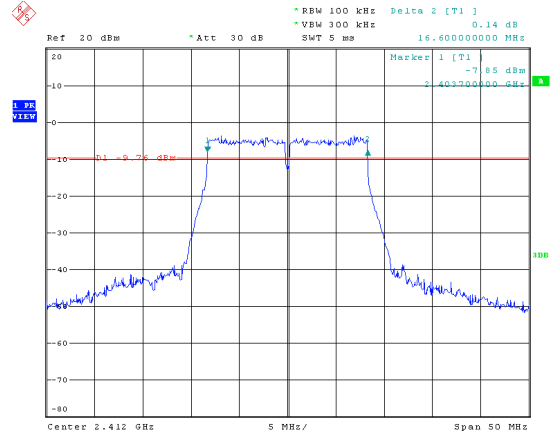
Modulation Type: 802.11g, ANT 0 CH01
