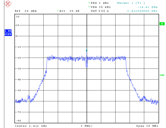
Modulation Type: 802.11g, ANT 1 CH01
