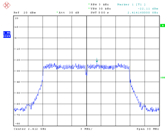
Modulation Type: 802.11n HT20, ANT 0 CH01
