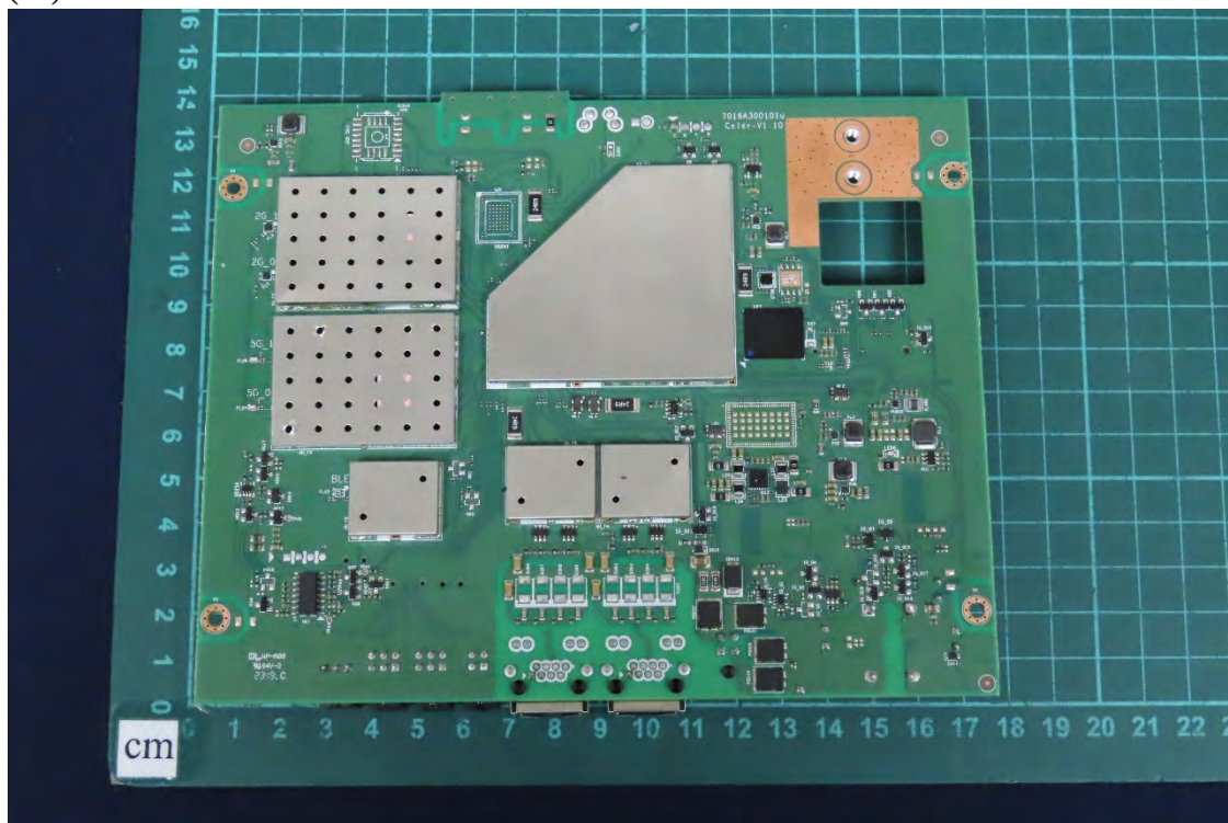
(32) EUT Photo
