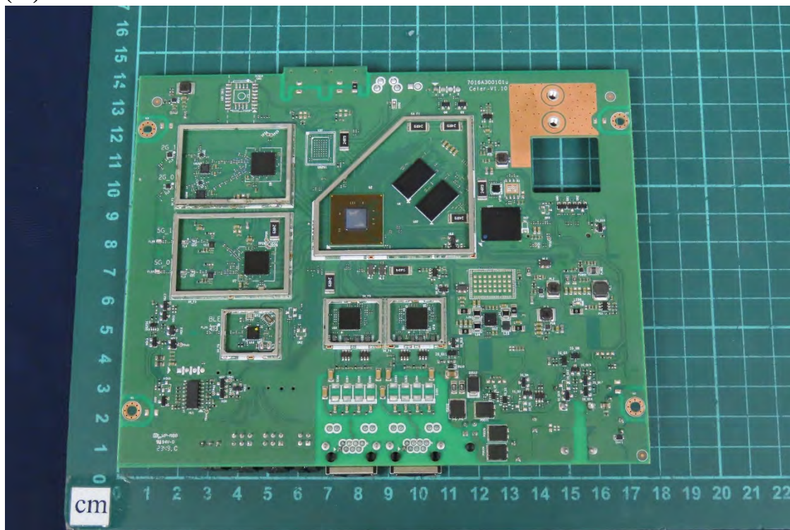
(34) EUT Photo
