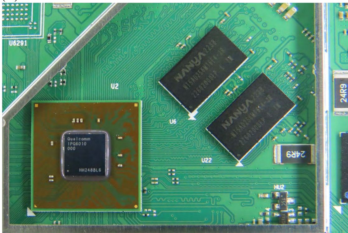
(39) EUT Photo
