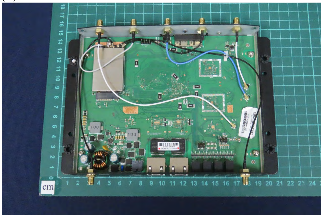
(25) EUT Photo
