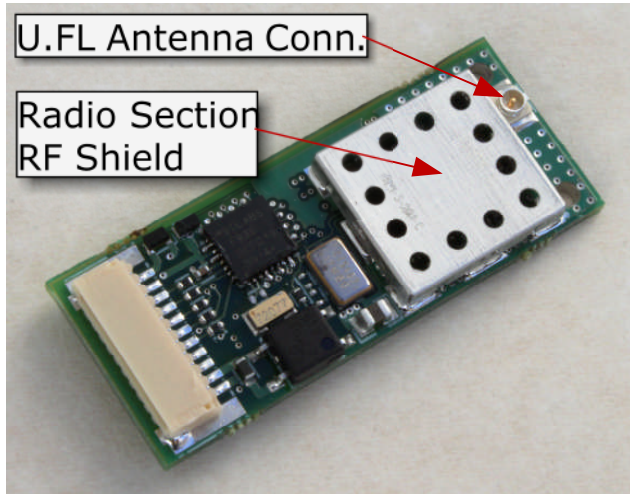
Model No. 10200 (top)
