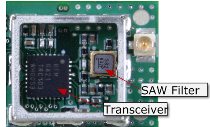
Radio section w/RF Shield removed
