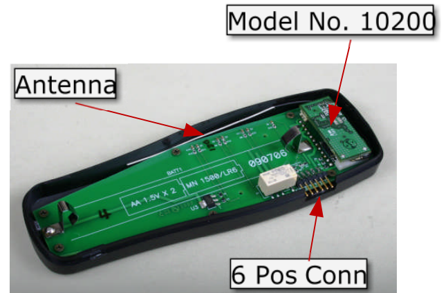
User Control (back removed)
