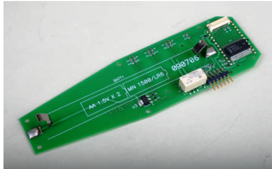
User Control Board (back)
