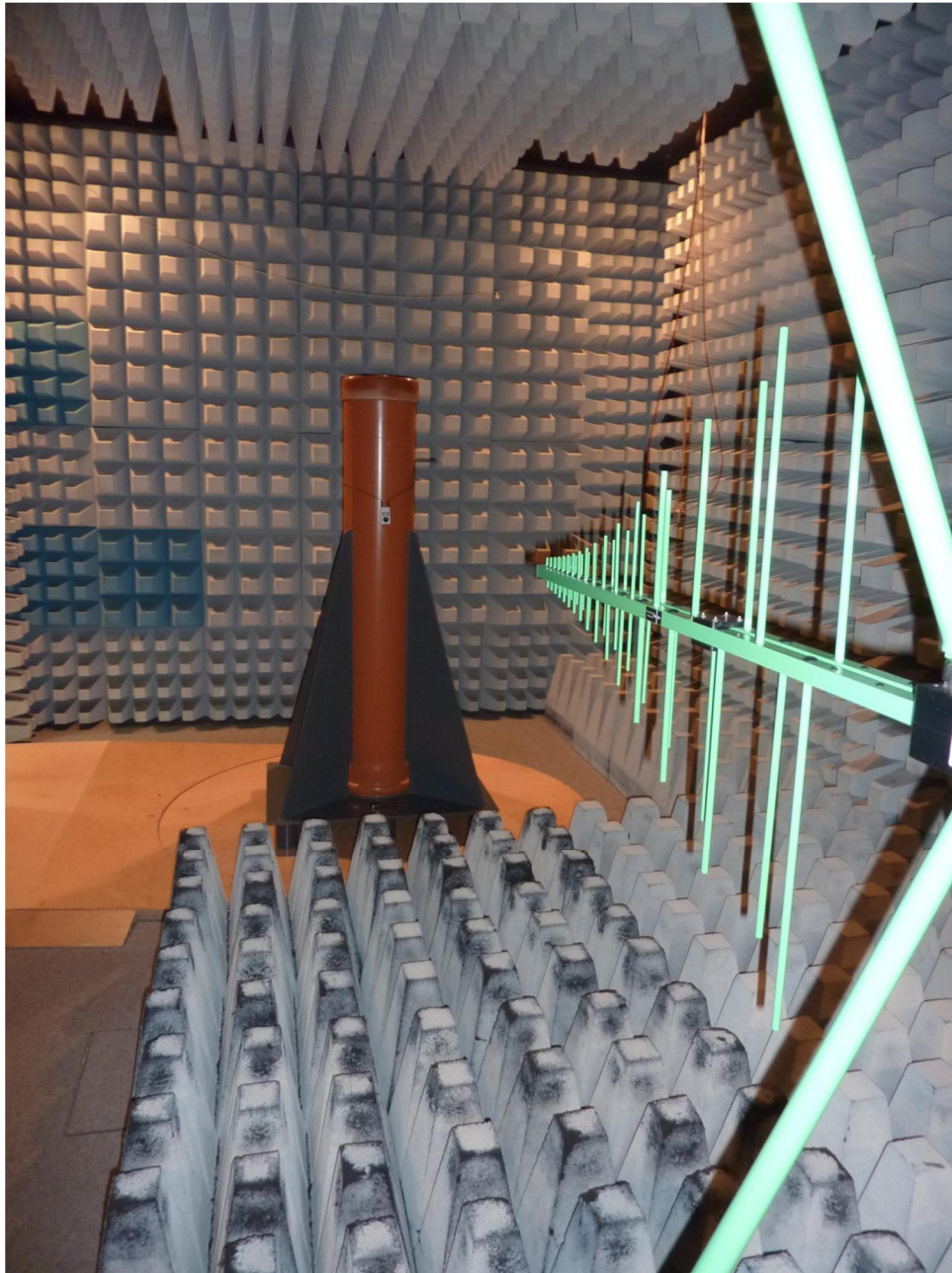
123800_05.JPG: Test setup fully anechoic chamber
