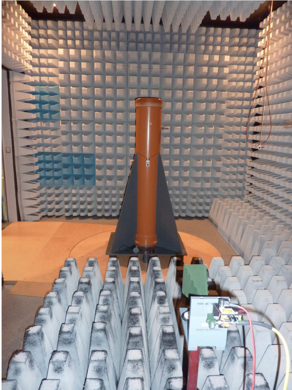
123800_10.JPG: Test setup fully anechoic chamber
