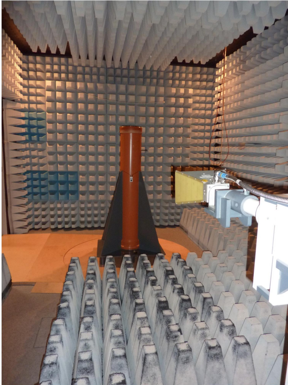
123800_12.JPG: Test setup fully anechoic chamber
