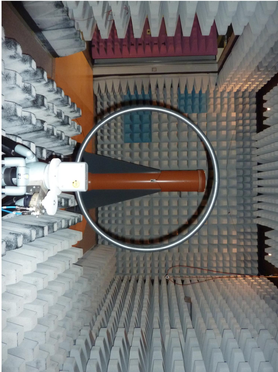
123800_13.JPG: Test setup fully anechoic chamber
