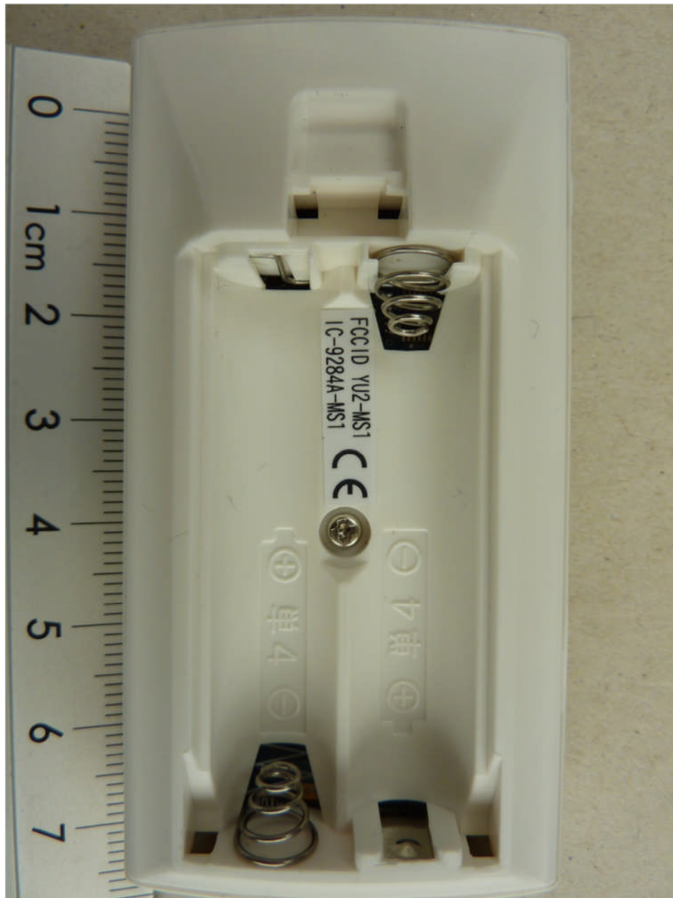
113324_41: Multistreamer, battery cover removed, label
