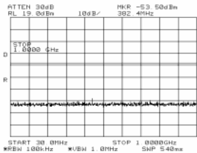
Antenna Port Emission Low Channel -1(802.11b)
