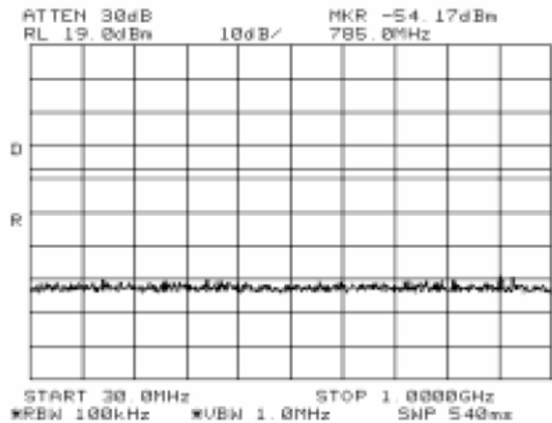
Antenna Port Emission High Channel-1 (802.11b)
