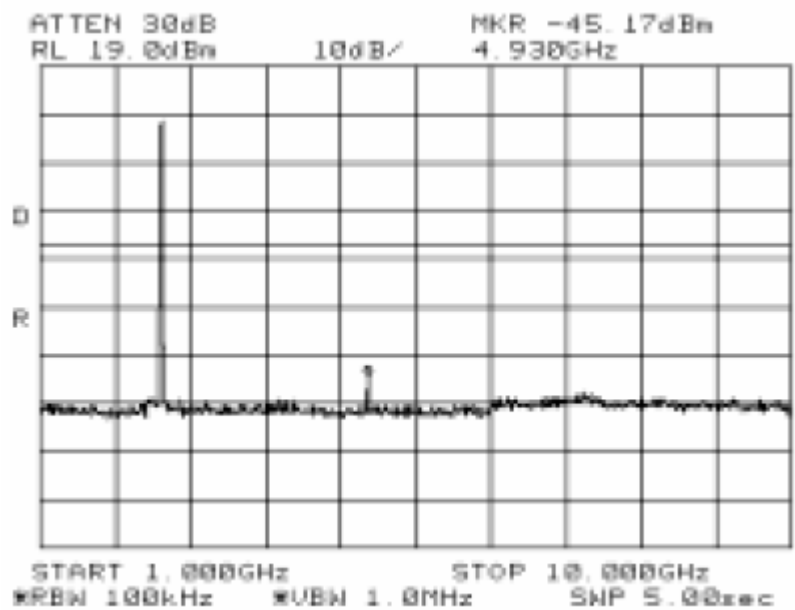
Antenna Port Emission High Channel-2 (802.11b)
