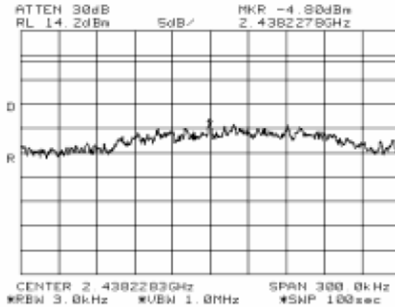
PSD - Mid Channel (802.11g)
