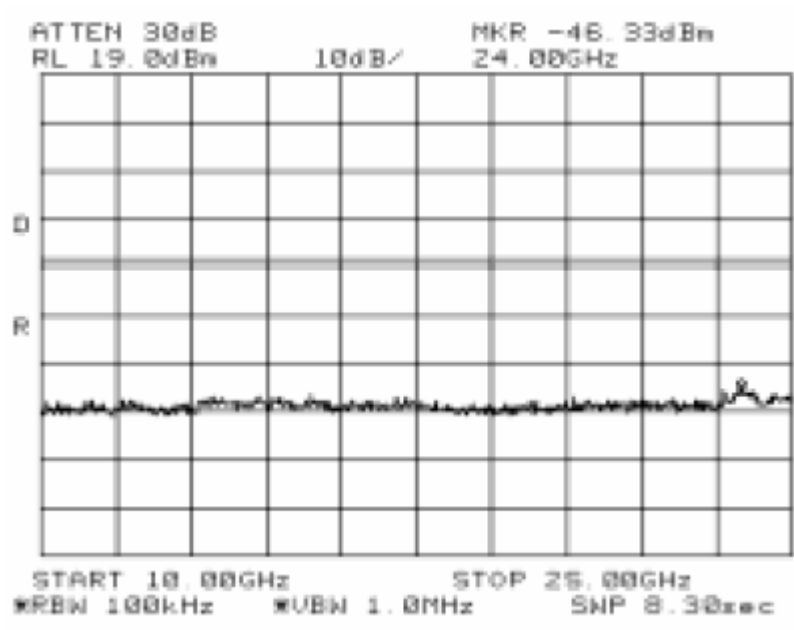
Antenna Port Emission Low Channel -3(802.11b)
