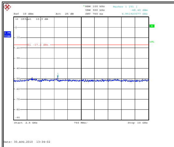
Figure 7.6.2.2-8: 2.5 GHz – 10 GHz – 2475MHz
