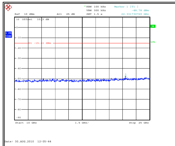
Figure 7.6.2.2-9: 10 GHz – 25 GHz – 2475MHz
