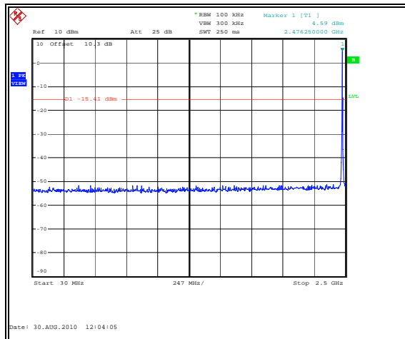
Figure 7.6.2.2-7: 30 MHz – 2.5 GHz – 2475MHz
