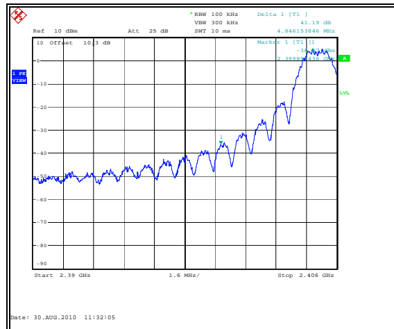
Figure 7.6.1.2-1: Lower Band-edge (Conducted)
