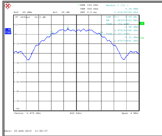
Figure 7.4.2-3: 6dB Bandwidth Plot – 2475MHz
