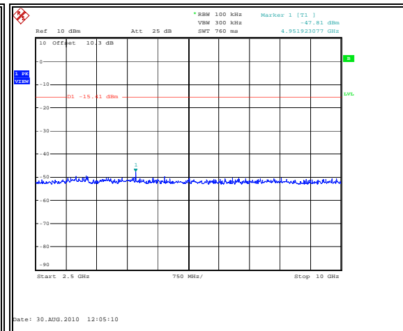
Figure 7.6.2.2-8: 2.5 GHz – 10 GHz – 2475MHz
