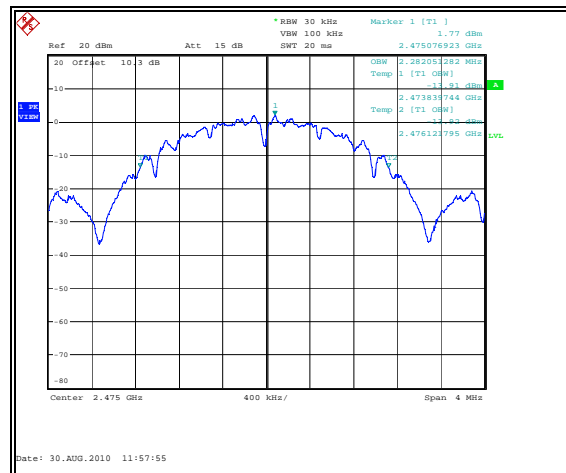
Figure 7.4.2-6: 99% Bandwidth Plot – 2475MHz
