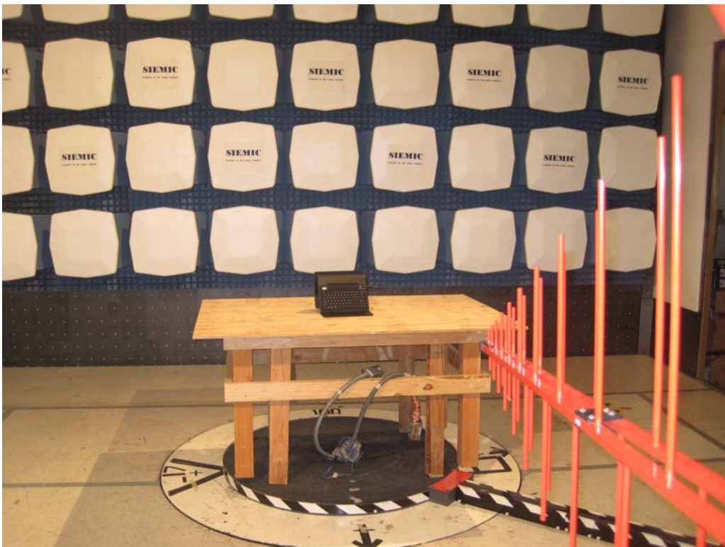
Radiated Emission (30MHz to 1GHz)- Rear View
