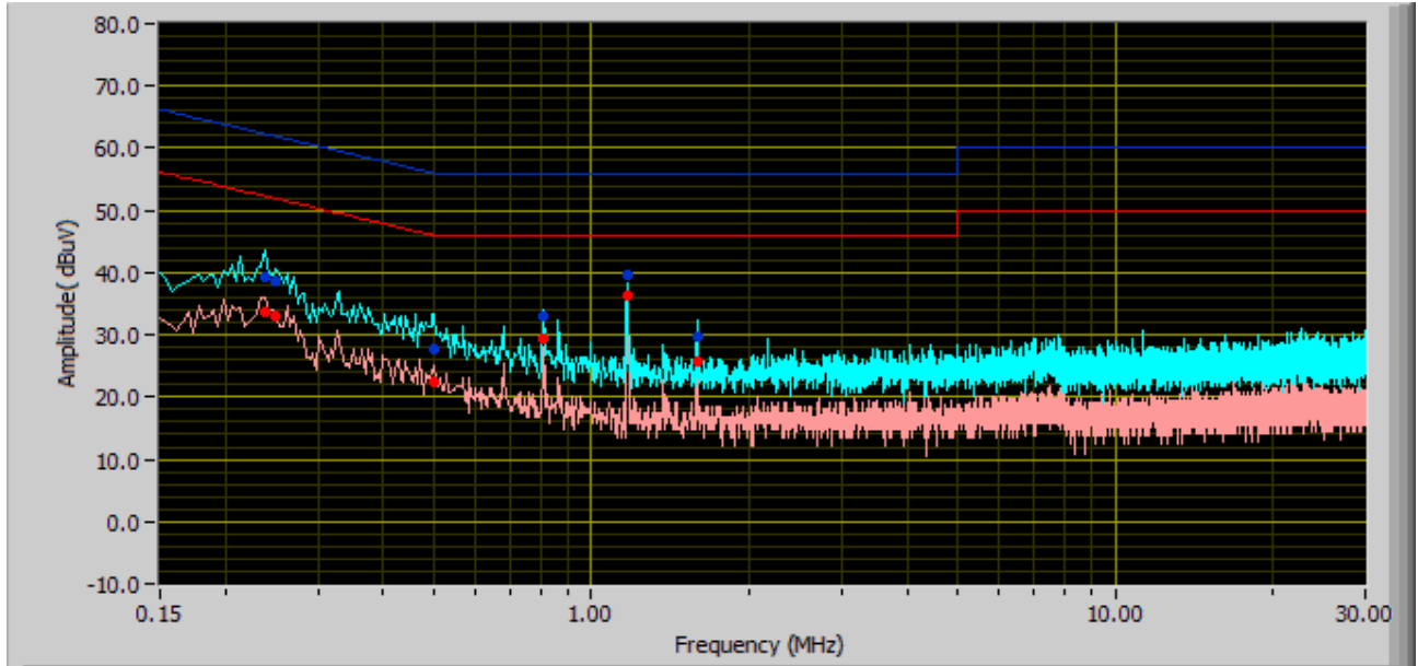
Phase Line Plot at 120VAC
