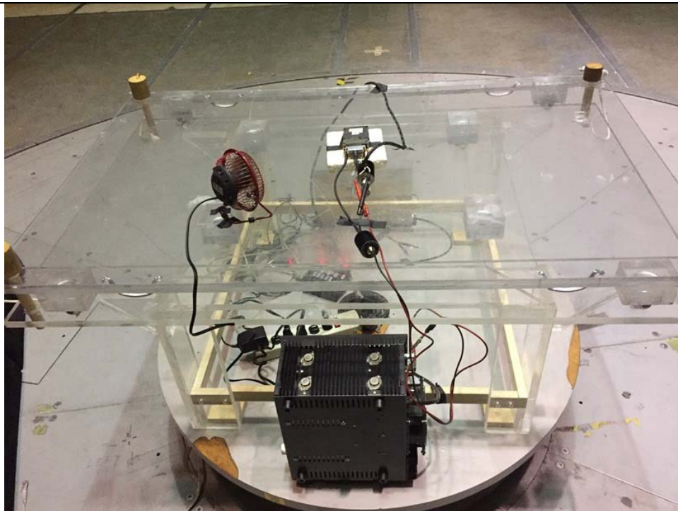
Radiated Emissions, Transmit Spurious, Back
