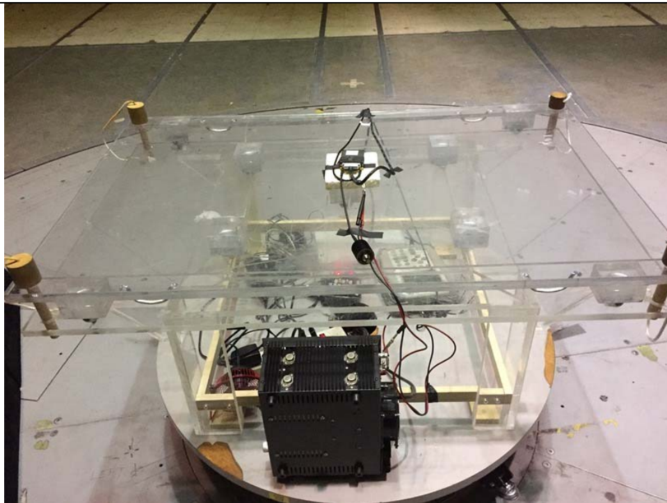
Radiated Emissions, Receive Mode, Back
