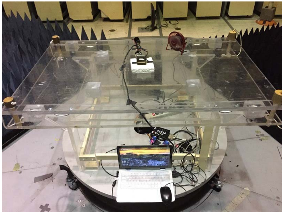
Radiated Emissions, Transmit Spurious, Front
