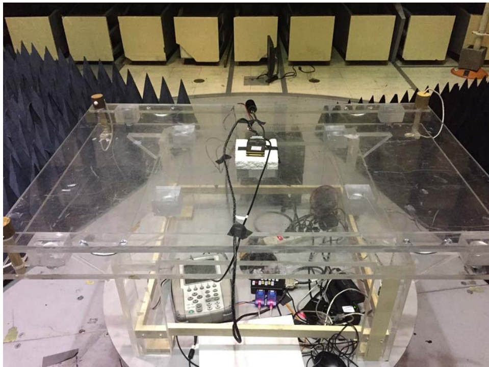
Radiated Emissions, Receive Mode, Front
