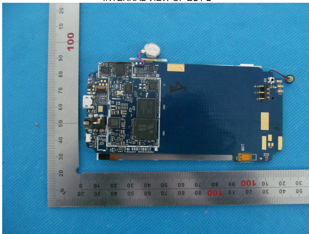
OPEN VIEW OF EUT_ (SINGLE SIM)
