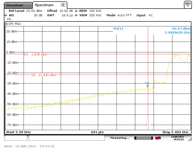
Hopping mode
