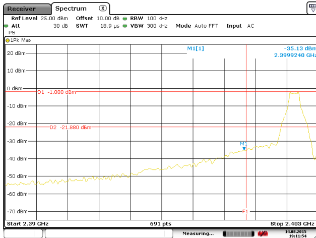
No-hopping mode
