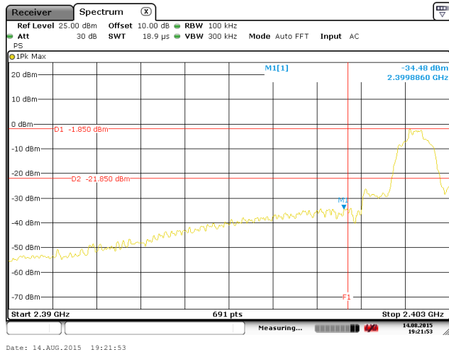
No-hopping mode
