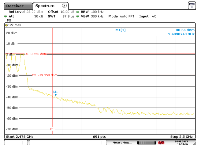
Hopping mode
