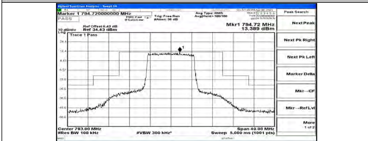
BAND 14_10MHz_16QAM
