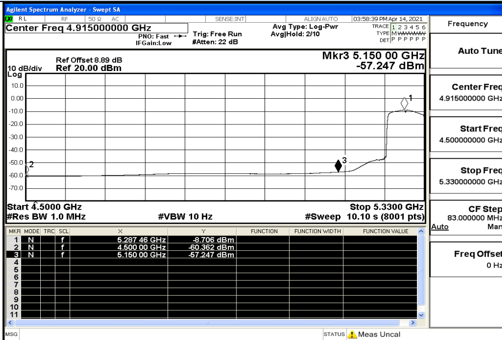
IEEE 802.11ac80 / Channel 42 / 5210MHz / Average
