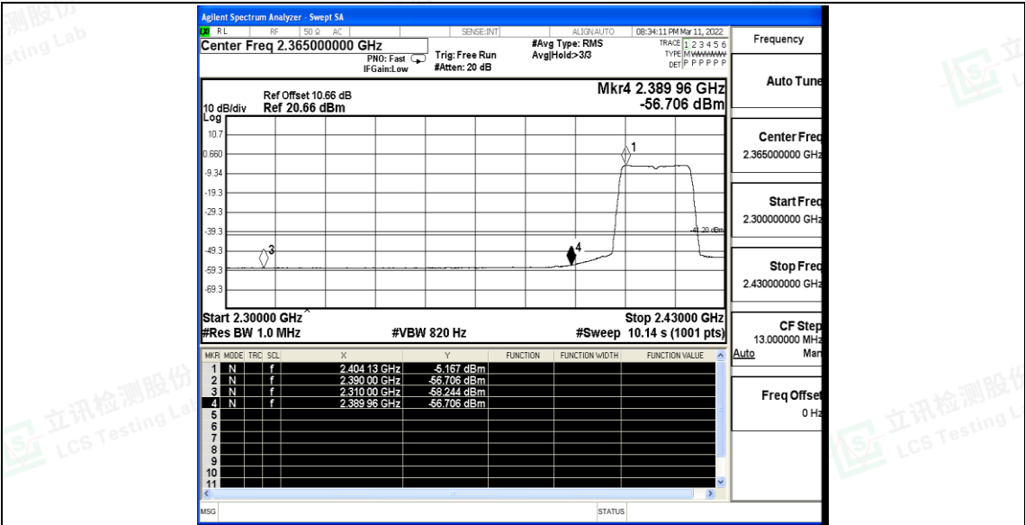
11N20SISO_Ant_Low_2412_Peak
