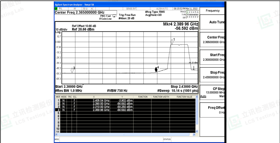
11G_Ant_Low_2412_Peak
