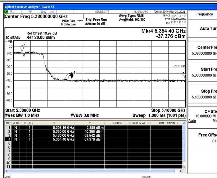
11AC40ISO_Ant1_High_5310_Peak
