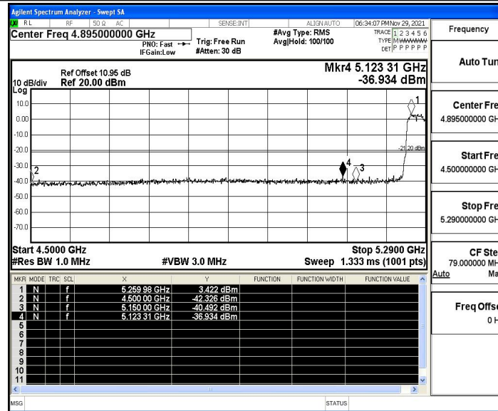
11AC40ISO_Ant1_High_5310_AV
