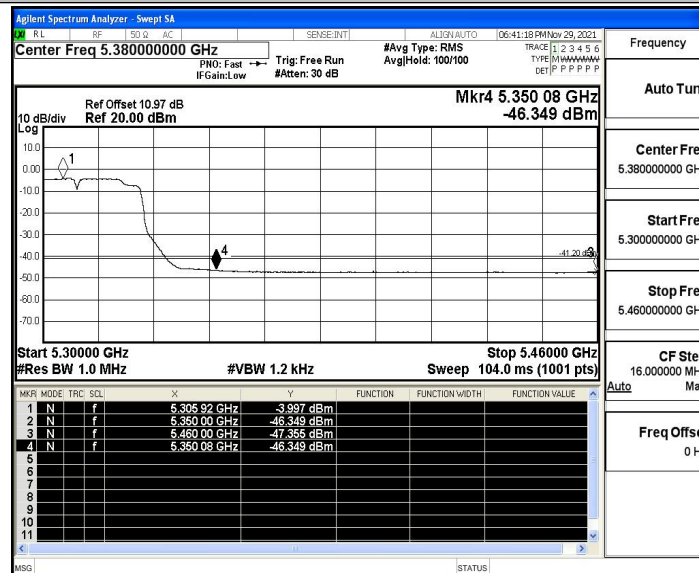
11AC40ISO_Ant1_High_5310_Peak
