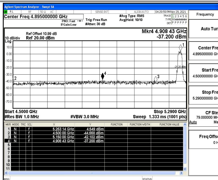
11N20SISO_Ant1_Low_5260_Peak
